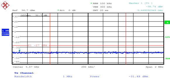
Diagram 8.5-6: Lower band edge, 802.11n HT40, ch1
