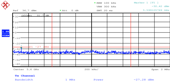
Diagram 8.5-18: Upper band edge of 5.6 GHz as per IC, 802.11n HT40, ch1
