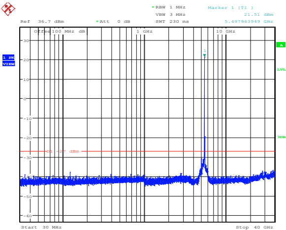
Diagram 8.5-25: Conducted spurious emissions for 802.11a, cho, low channel
