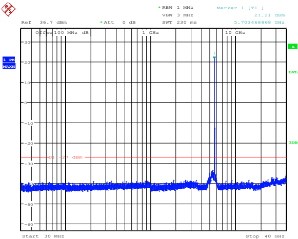
Diagram 8.5-29: Conducted spurious emissions for 802.11n HT40, cho, low channel
