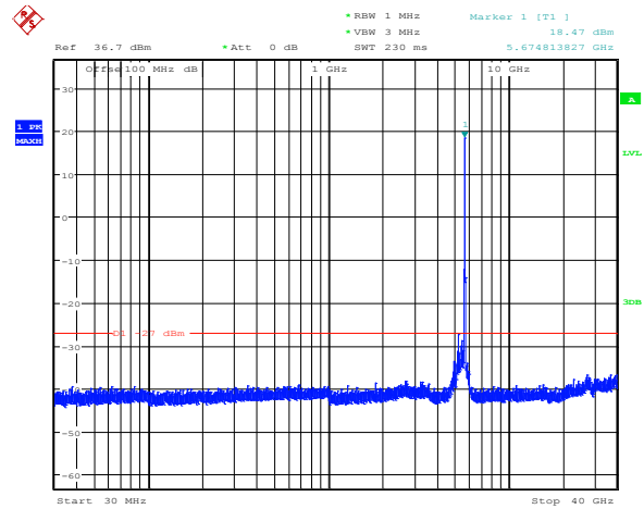
Diagram 8.5-34: Conducted spurious emissions for 802.11n HT20, ch1, high channel
