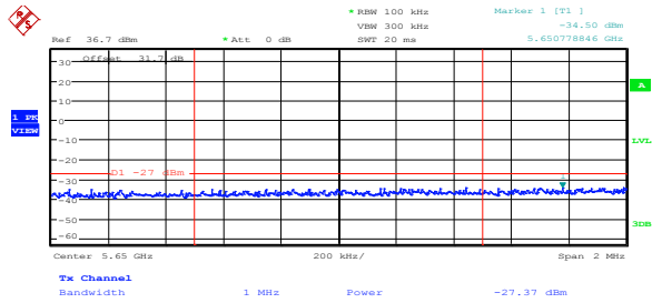
Diagram 8.5-23: Lower band edge of 5.65 GHz as per IC, 802.11n HT40, cho
