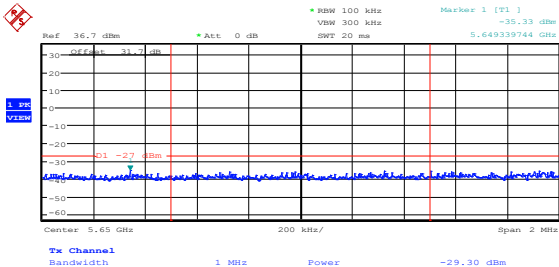
Diagram 8.5-14: Upper band edge of 5.6 GHz as per IC, 802.11a, ch1
