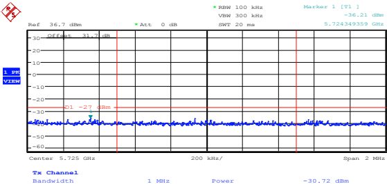
Diagram 8.5-8: Upper band edge, 802.11a, ch1
