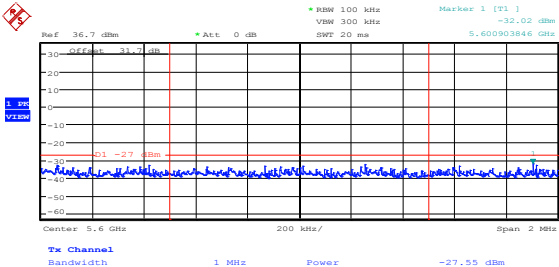
Diagram 8.5-17: Upper band edge of 5.6 GHz as per IC, 802.11n HT40, cho
