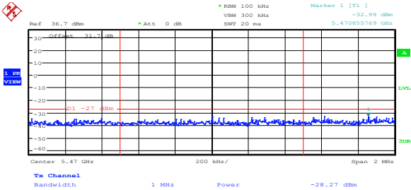
Diagram 8.5-3: Lower band edge, 802.11n HT20, cho
