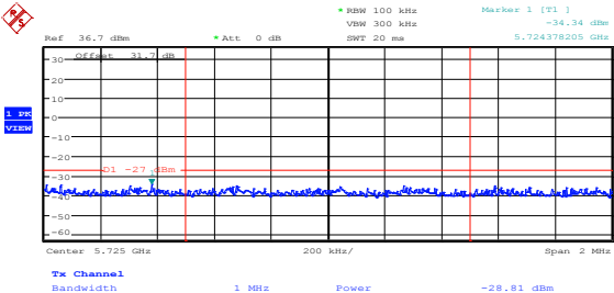
Diagram 8.5-12: Upper band edge, 802.11n HT40, ch1
