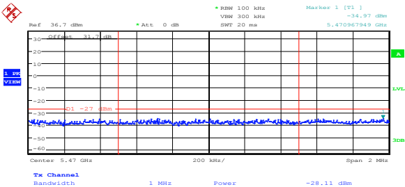
Diagram 8.5-5: Lower band edge, 802.11n HT40, cho
