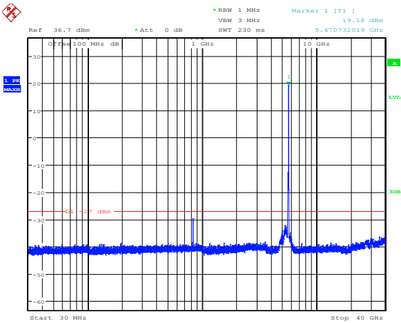
Diagram 8.5-33: Conducted spurious emissions for 802.11n HT20, cho, high channel
