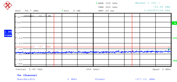
Diagram 8.5-24: Lower band edge of 5.65 GHz as per IC, 802.11n HT40, ch1
