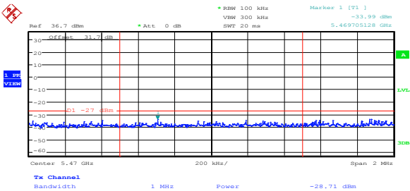
Diagram 8.5-1: Lower band edge, 802.11a, cho
