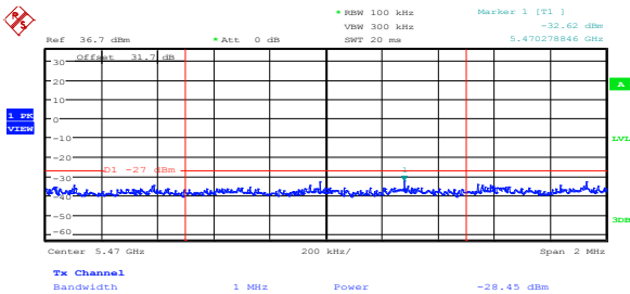
Diagram 8.5-2: Lower band edge, 802.11a, ch1
