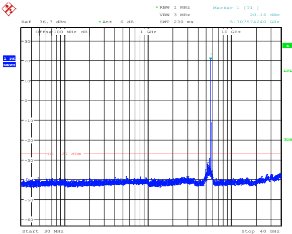
Diagram 8.5-30: Conducted spurious emissions for 802.11n HT40, ch1, low channel
