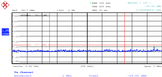
Diagram 8.5-16: Upper band edge of 5.6 GHz as per IC, 802.11n HT20, ch1
