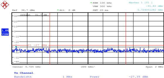
Diagram 8.5-11: Upper band edge, 802.11n HT40, cho
