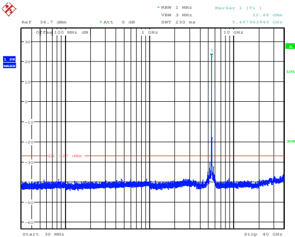
Diagram 8.5-26: Conducted spurious emissions for 802.11a, ch1, low channel
