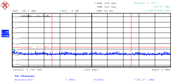
Diagram 8.5-7: Upper band edge, 802.11a, cho
