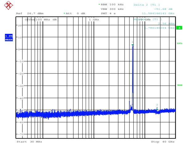
Diagram 8.5-6: Conducted spurious emissions for 802.11a, cho, high channel
