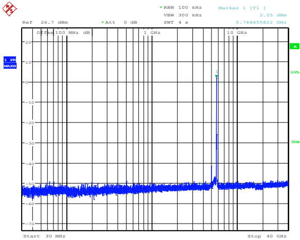
Diagram 8.5-1: Conducted spurious emissions for 802.11a, cho, low channel
