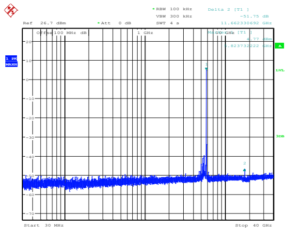
Diagram 8.5-13: Conducted spurious emissions for 802.11n HT20, ch1, mid channel
