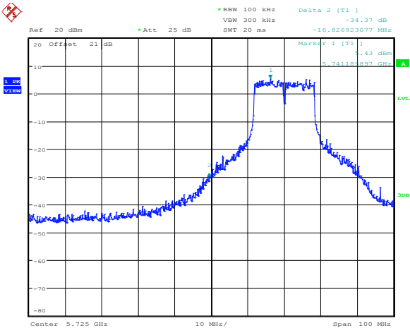
Diagram 8.5-17: Lower band edge emissions for 802.11a, cho
