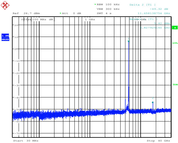
Diagram 8.5-5: Conducted spurious emissions for 802.11n HT20, cho, mid channel
