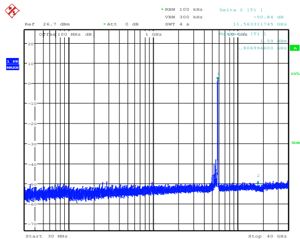
Diagram 8.5-14: Conducted spurious emissions for 802.11a, ch1, high channel
