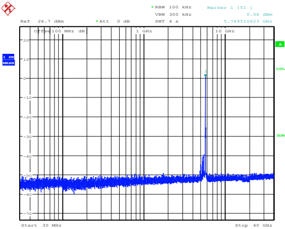
Diagram 8.5-9: Conducted spurious emissions for 802.11a, ch1, low channel
