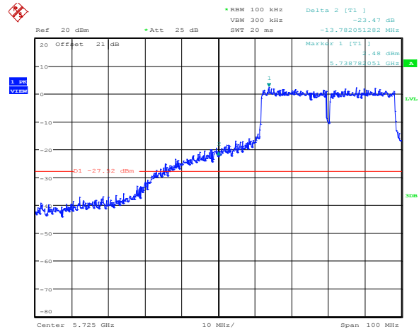
Diagram 8.5-22: Lower band edge emissions for 802.11n HT40, ch1
