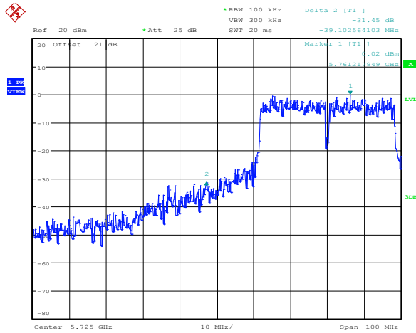
Diagram 8.5-21: Lower band edge emissions for 802.11n HT40, cho
