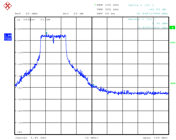
Diagram 8.5-24: Upper band edge emissions for 802.11a, cho
