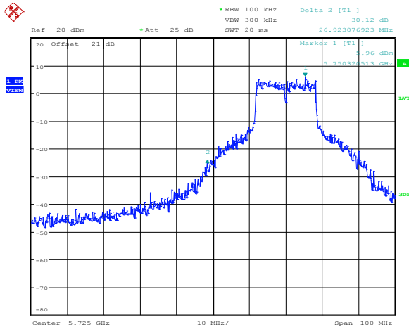
Diagram 8.5-18: Lower band edge emissions for 802.11a, ch1
