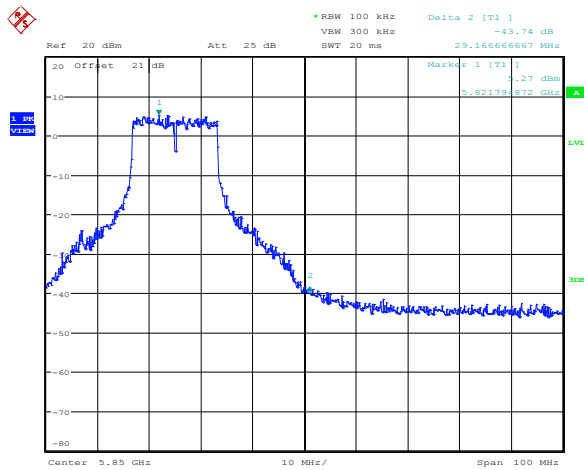
Diagram 8.5-23: Upper band edge emissions for 802.11a, cho
