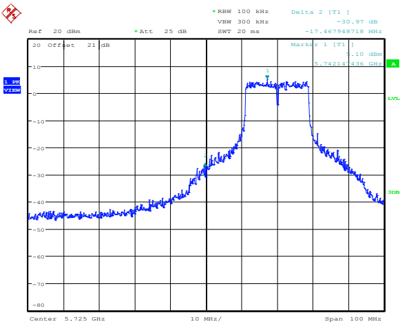
Diagram 8.5-19: Lower band edge emissions for 802.11n HT20, cho
