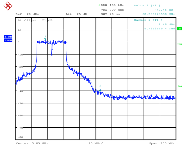
Diagram 8.5-29: Upper band edge emissions for 802.11n HT40, cho
