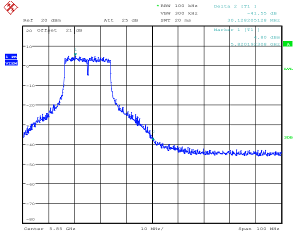
Diagram 8.5-26: Upper band edge emissions for 802.11n HT20, cho
