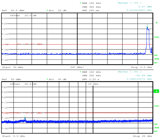
Figure 8.5-14: Conducted spurious emissions for 802.11g, ch1, low channel
