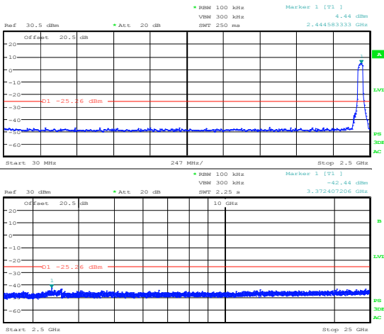
Figure 8.5-6: Conducted spurious emissions for 802.11g, cho, mid channel
