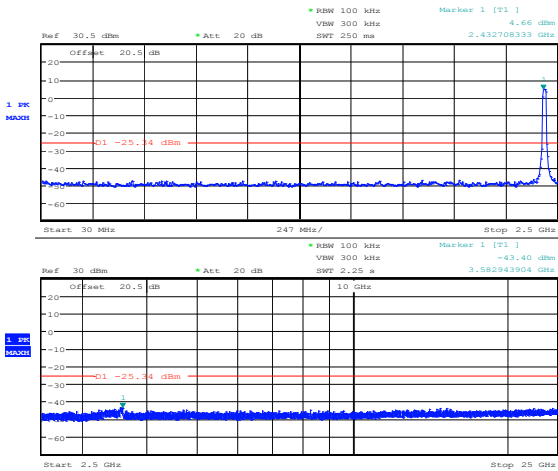
Figure 8.5-5: Conducted spurious emissions for 802.11b, cho, mid channel
