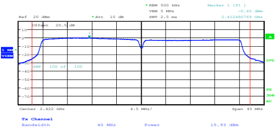
Figure 8.4-4: Output power on 802.11n HT40, sample plot
