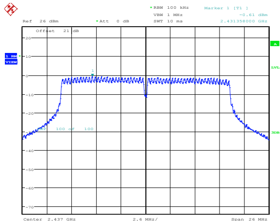
Figure 8.6-3: PSD sample plot on 802.11n HT20
