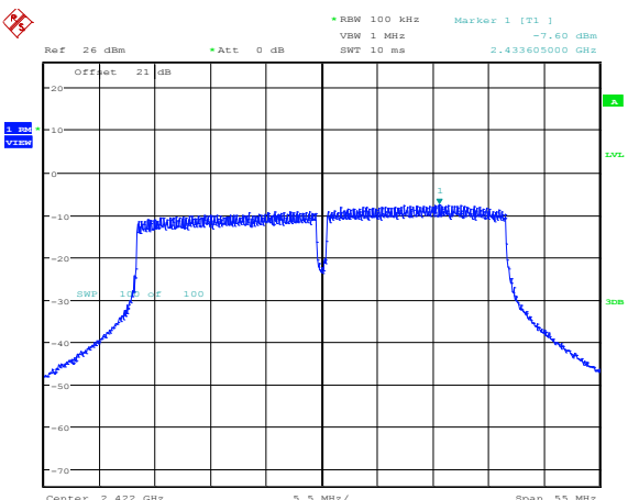
Figure 8.6-4: PSD sample plot on 802.11n HT40
