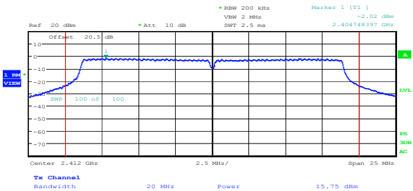
Figure 8.4-3: Output power on 802.11n HT20, sample plot
