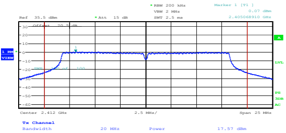
Figure 8.4-2: Output power on 802.11g, sample plot
