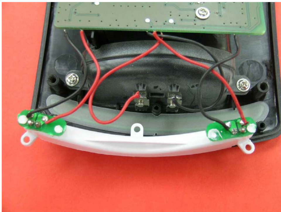
Base LED PCB rear side
