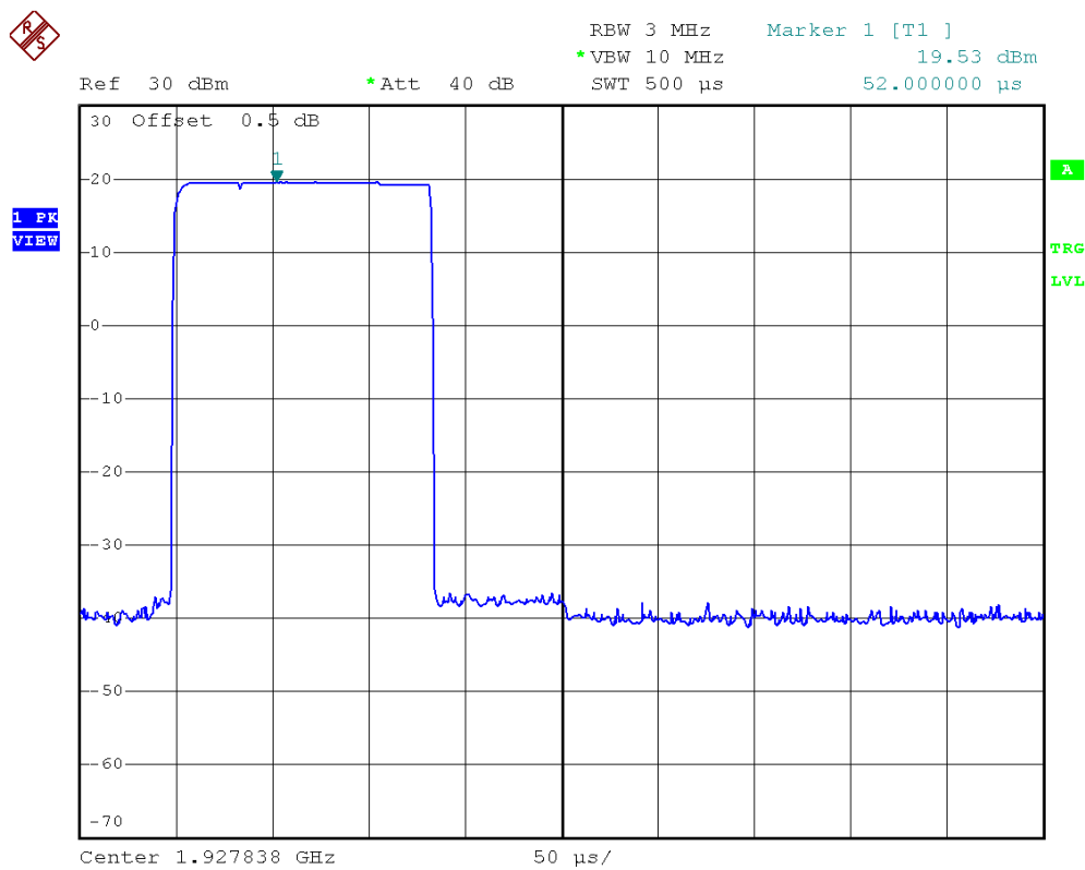
Plot 2D. Highest Channel Peak Transmit Power (Dummy Carrier)
