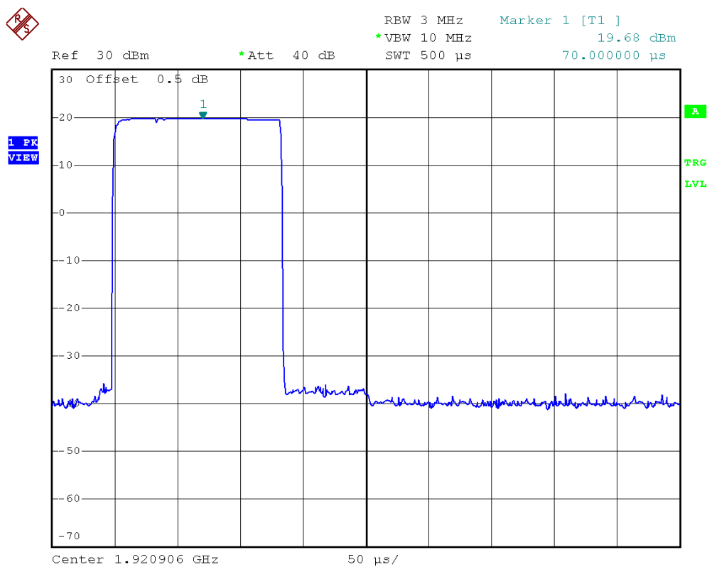
Plot 2C. Lowest Channel Peak Transmit Power (Dummy Carrier)
