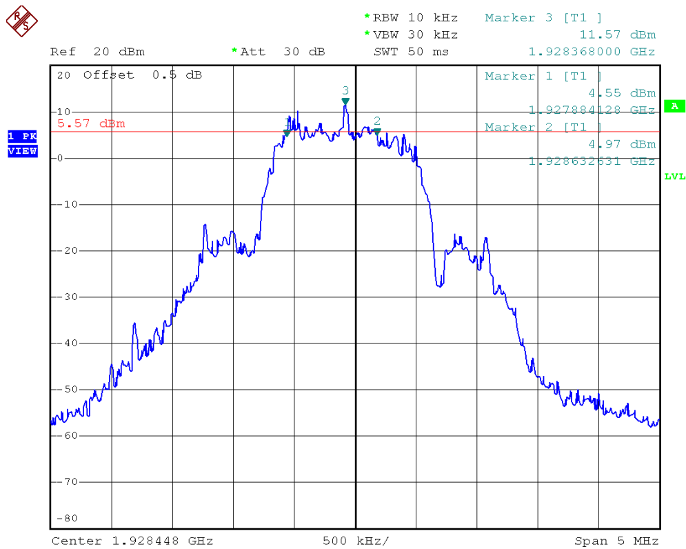
Plot 1E. Highest Channel Test Frequency at -6dB points (Traffic Carrier)
