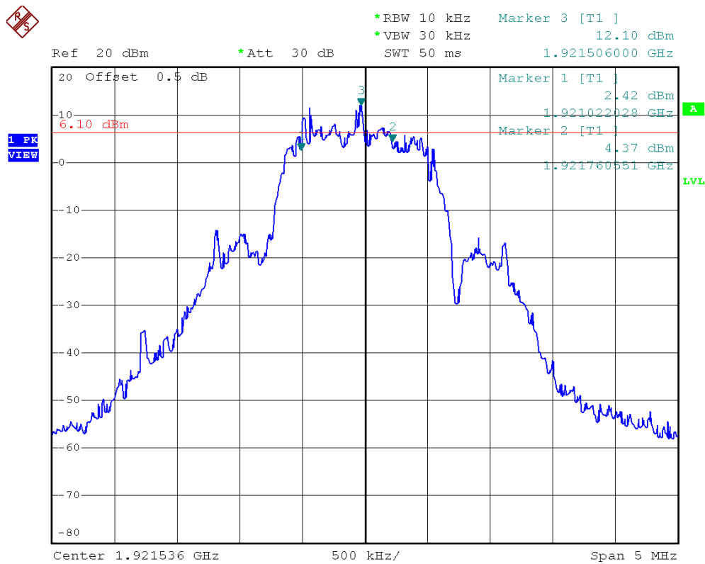
Plot 1B. Lowest Channel Test Frequency at -6dB points (Traffic Carrier)
