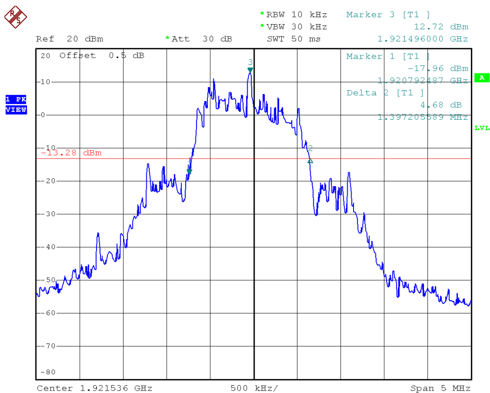
Plot 1G. Lowest Channel 26dB Emission Bandwidth (Dummy Carrier)
