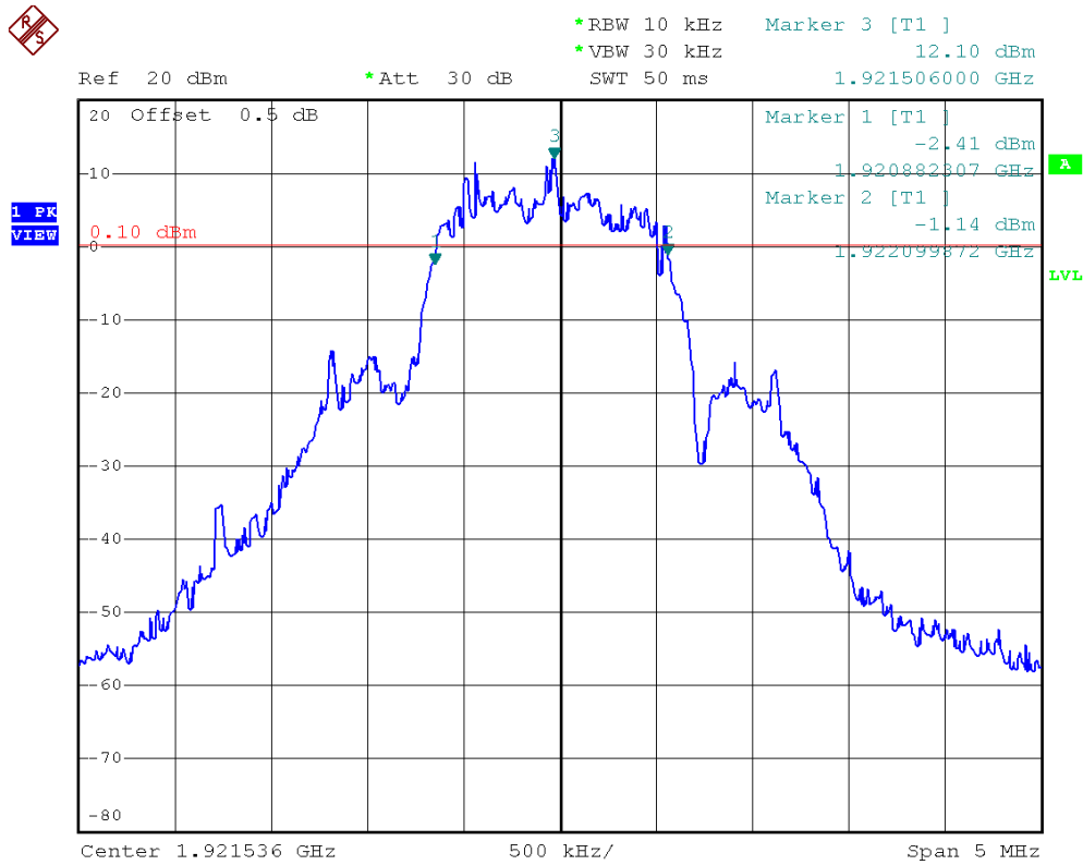
Plot 1C. Lowest Channel Test Frequency at -12dB points (Traffic Carrier)
