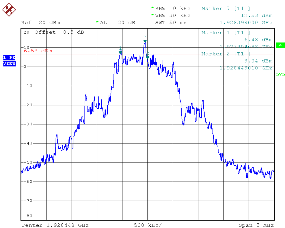
Plot 1K. Highest Channel Test Frequency at -6dB points (Dummy Carrier)
