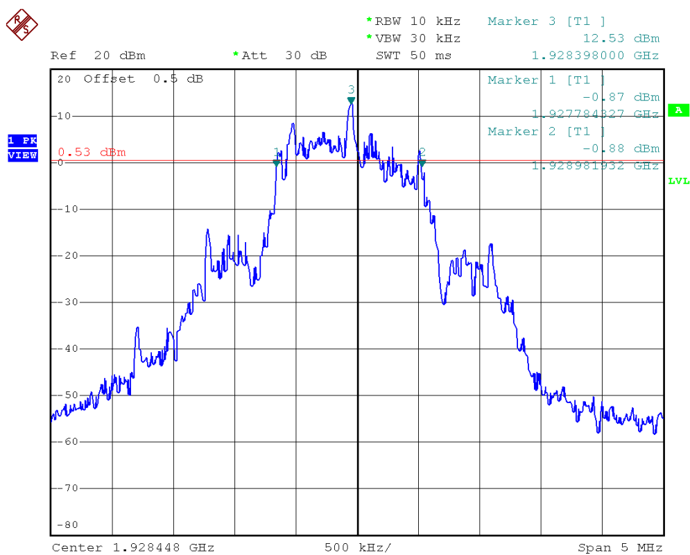
Plot 1L. Highest Channel Test Frequency at -12dB points (Dummy Carrier)
