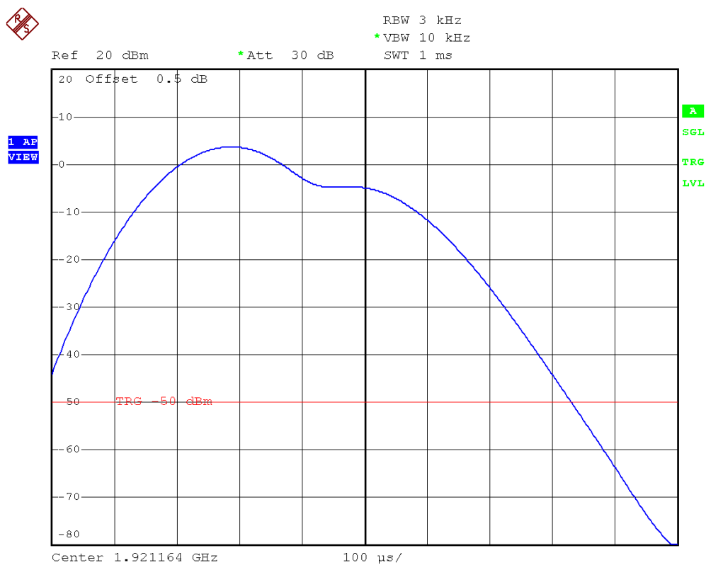
Plot 3A. Lowest Channel Power Spectral Density (Traffic Carrier)
