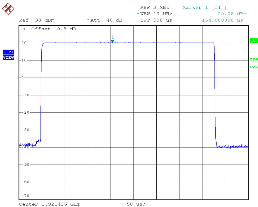
Plot 2A. Lowest Channel Peak Transmit Power (Traffic Carrier)
