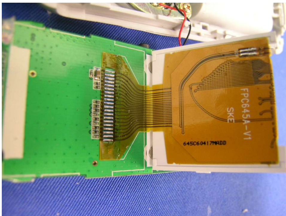
Handset Main PCB display side (View 4)
