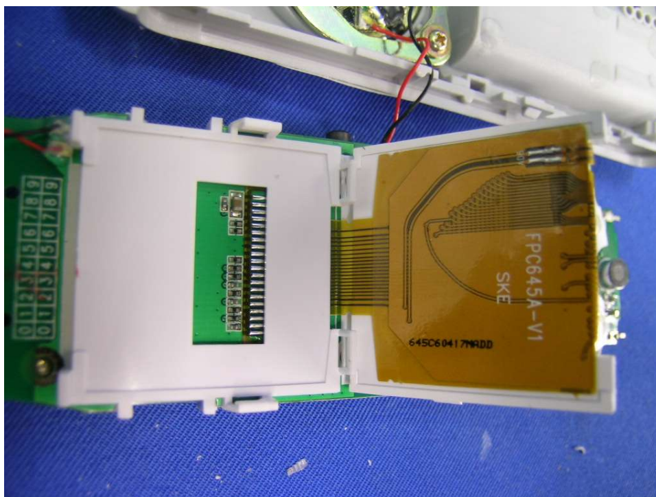
Handset Main PCB display side (View 3)
