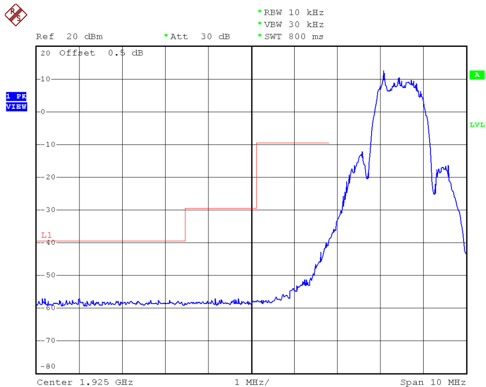
Plot 4B. Highest Channel Unwanted Emission Inside the Sub-Band (Traffic Carrier)
