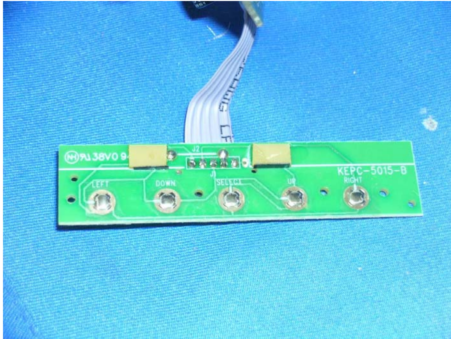
Wireless caller ID display unit keypad front side
