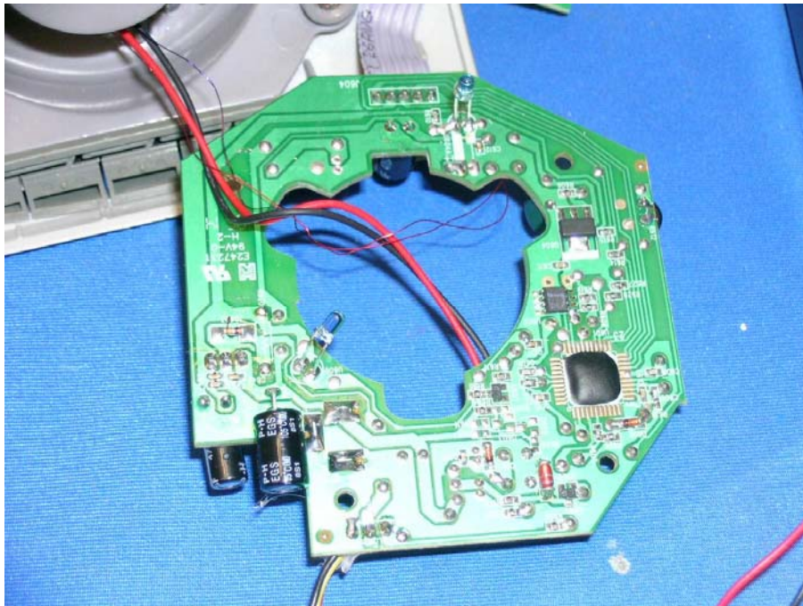
Wireless caller ID display Unit Main PCB front side
