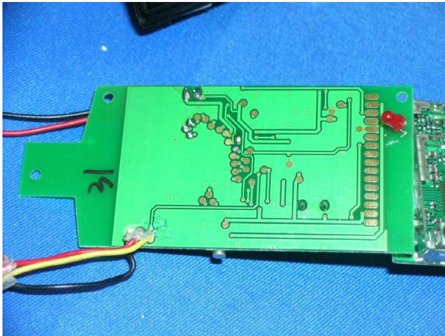
Wireless caller ID display Unit another PCB solder side
