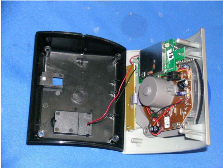
Wireless caller ID display unit assembly
