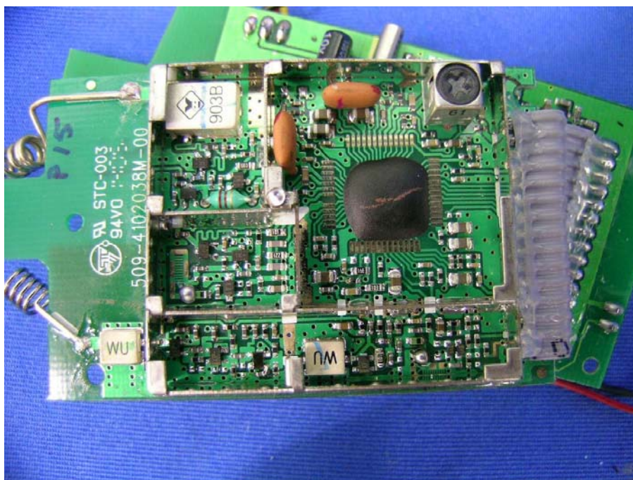
Wireless caller ID display Unit Oscillator PCB comp side
