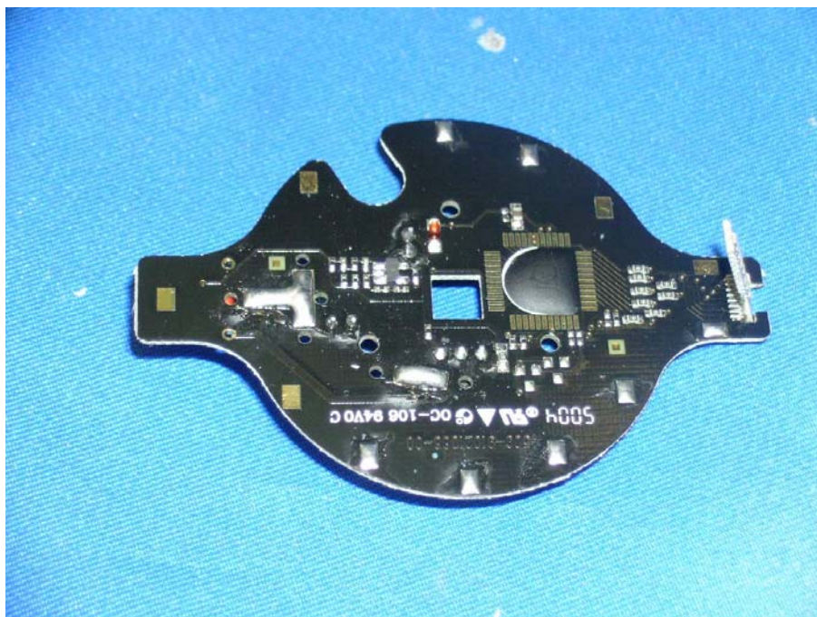
Wireless caller ID display Unit Rotator PCB rear side
