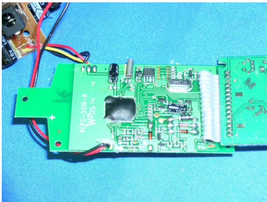
Wireless caller ID display Unit another PCB comp side (View 1)
