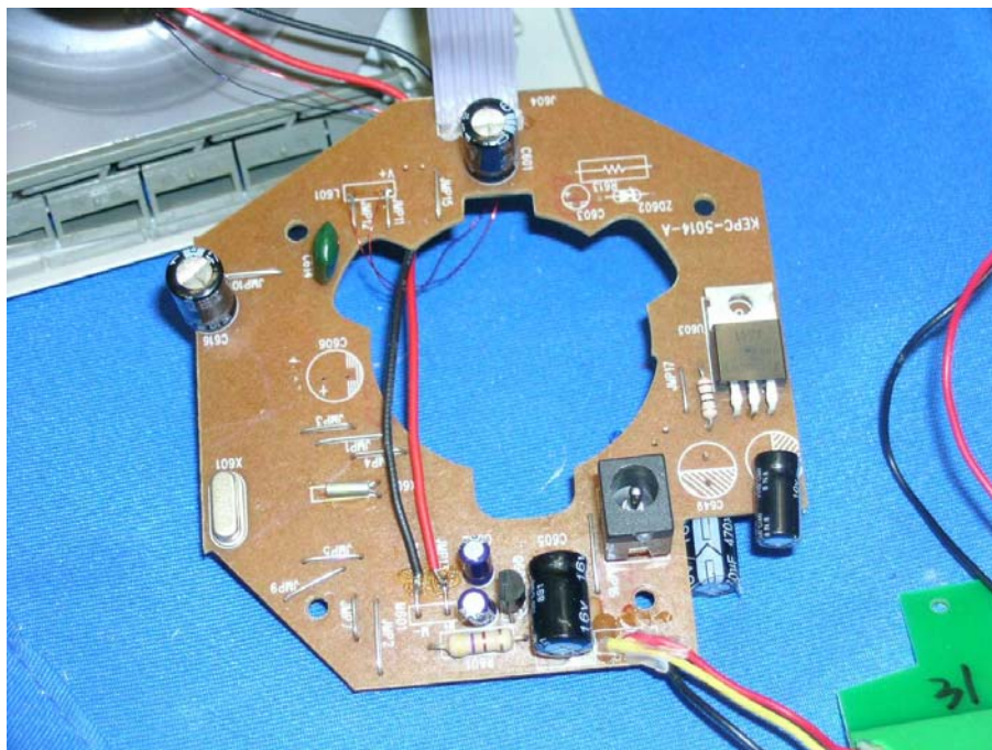
Wireless caller ID display Unit Main PCB rear side
