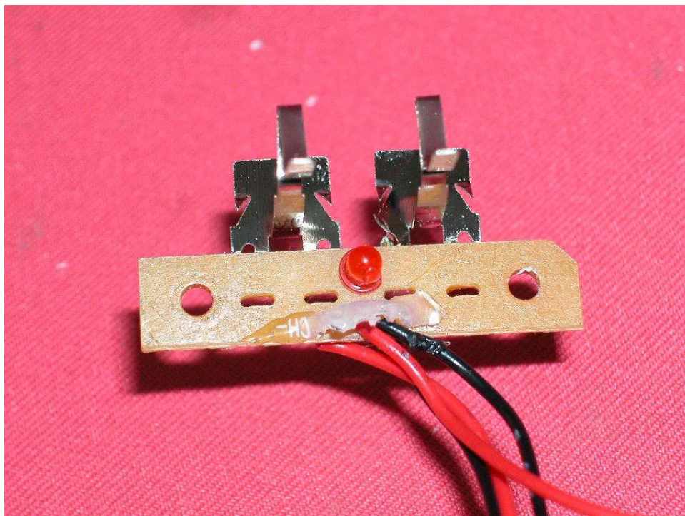
Base Charging LED front side
