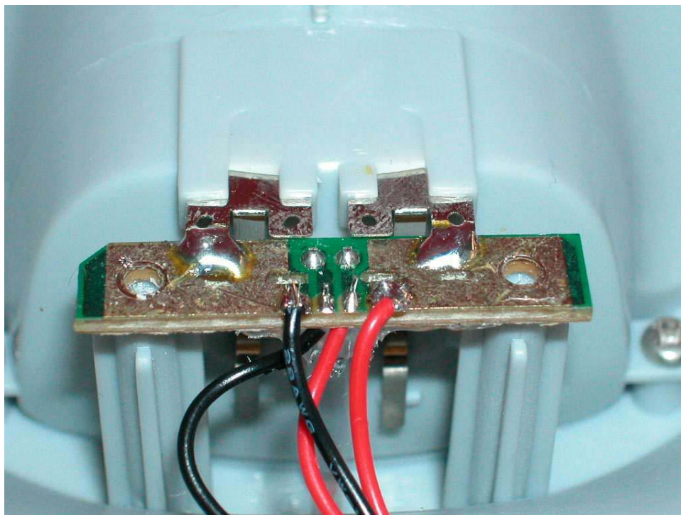
Base Charging LED rear side
