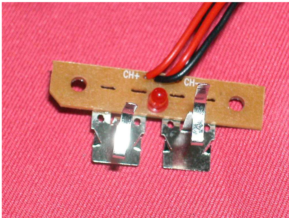
Base charging PCB front side
