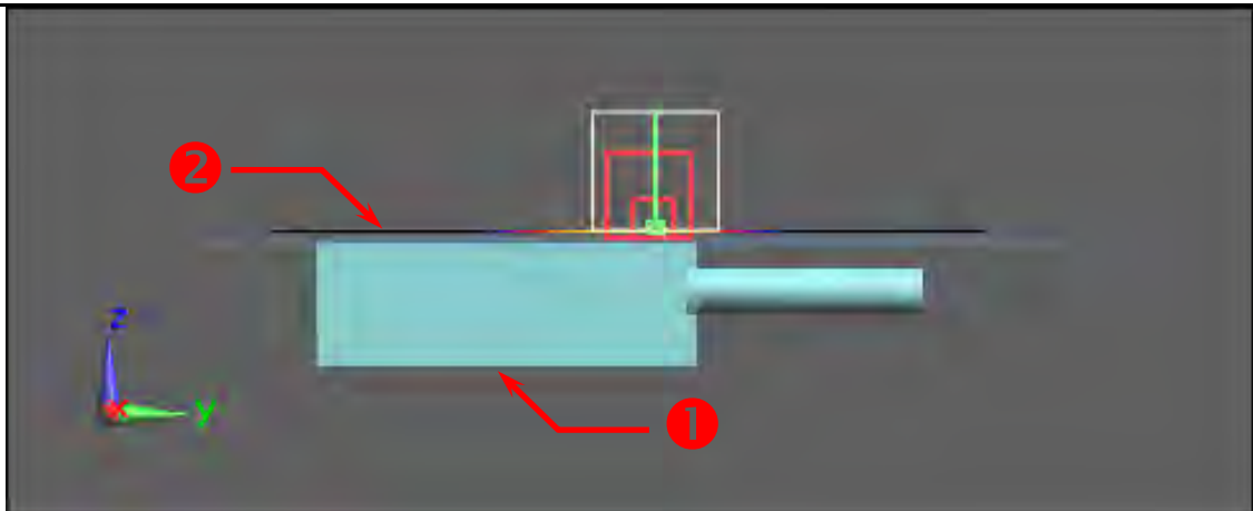
Figure 4. Body SAR Test Setup (Flat Section)
