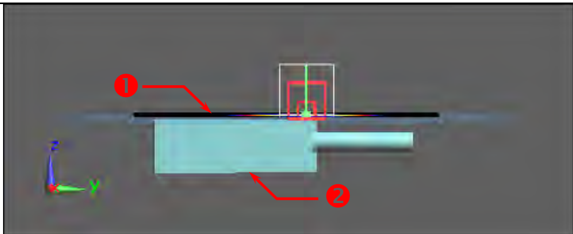
Figure 2. Body SAR Test Setup (Flat Section)
