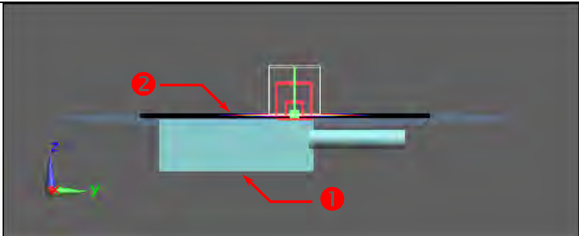
Figure 3. Body SAR Test Setup (Flat Section)
