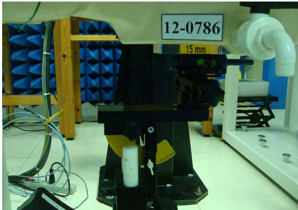
Figure 3. Body SAR Test Setup (Flat Section)
