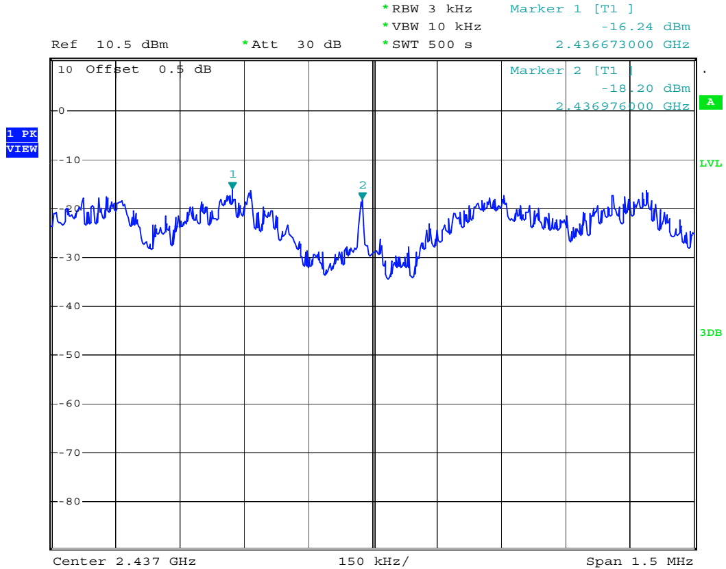
Plot: G3B1 (6Mbps)
