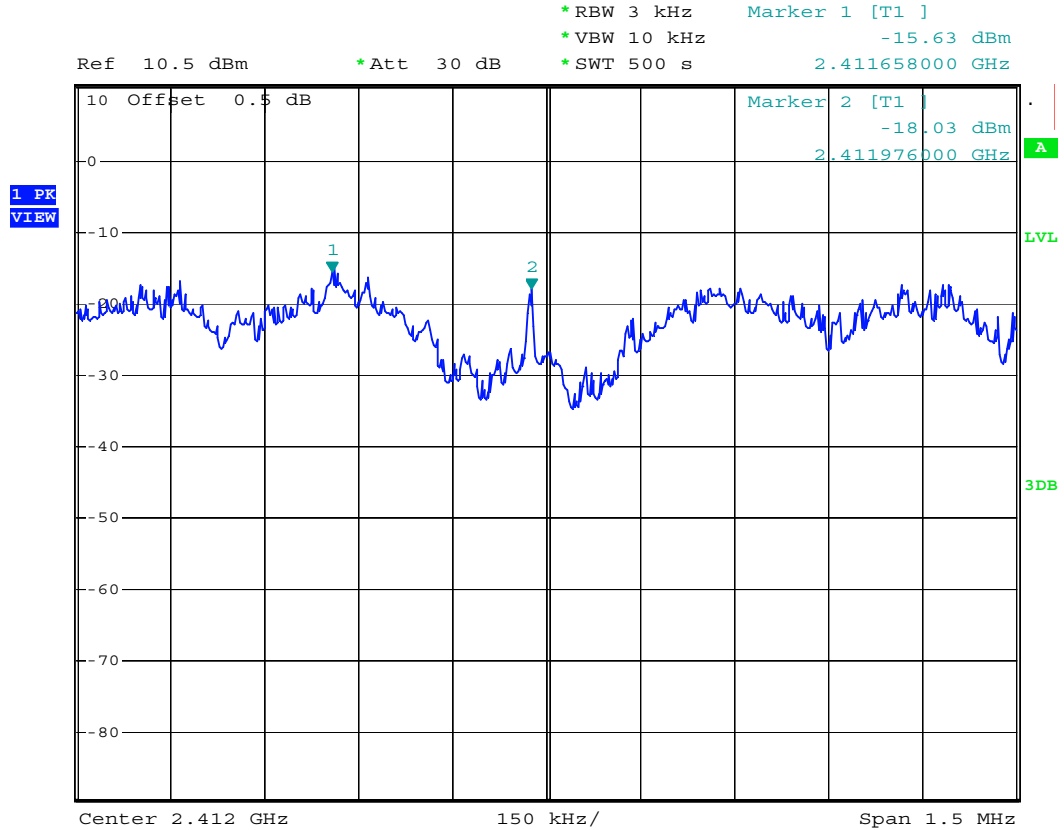
Plot: G3A1 (6Mbps)
