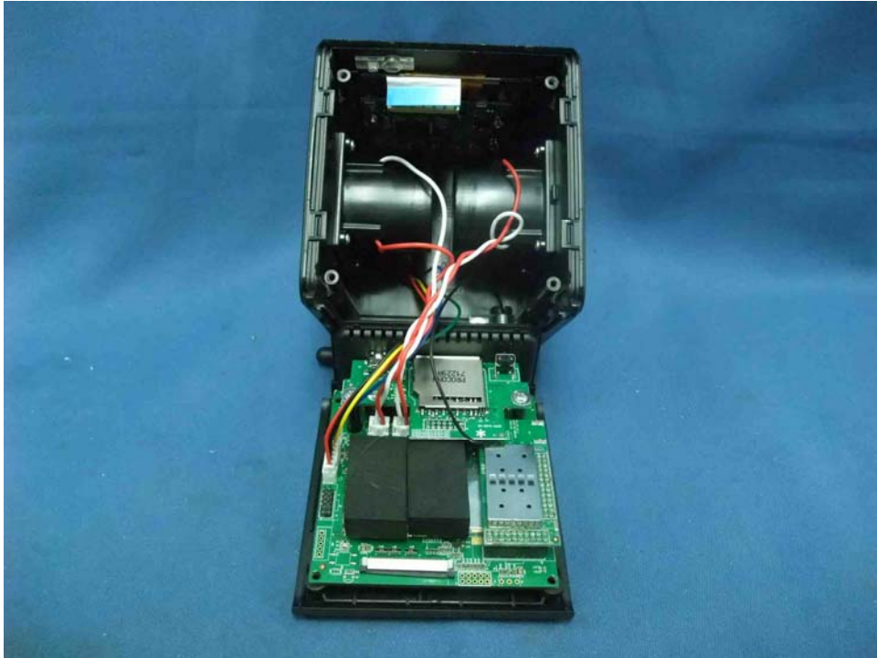
WiFi Internal Radio Player assembly
