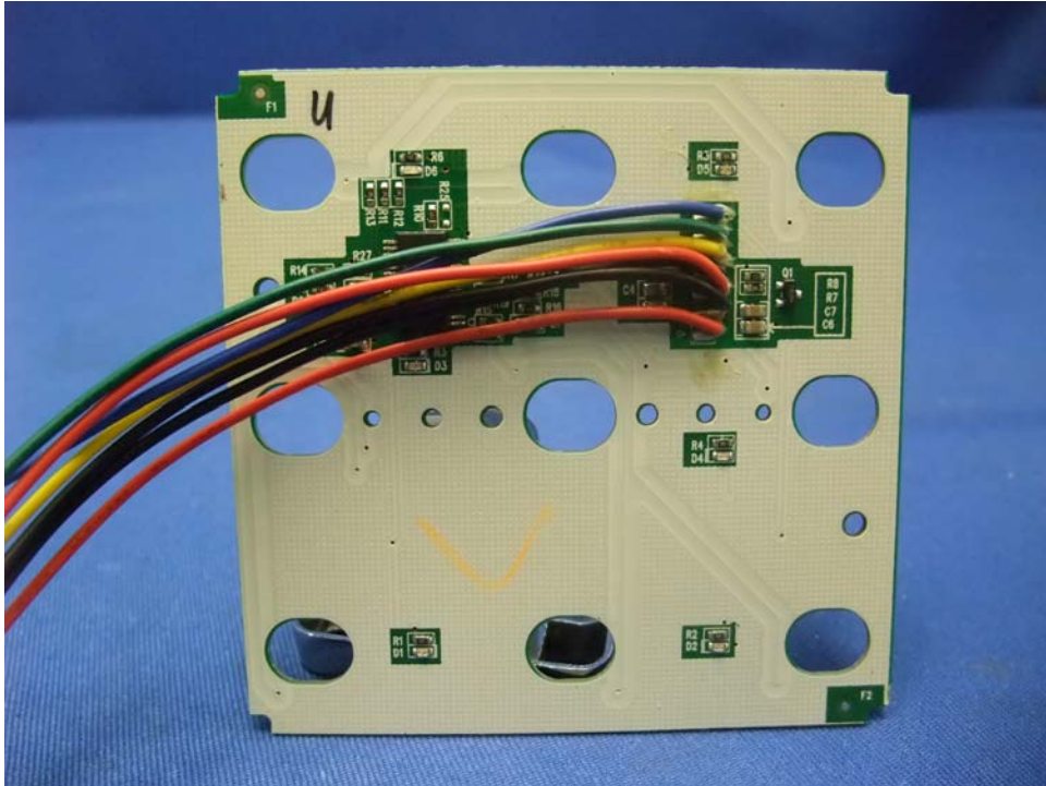
WiFi Internal Radio Player Keyboard front side (View 2)
