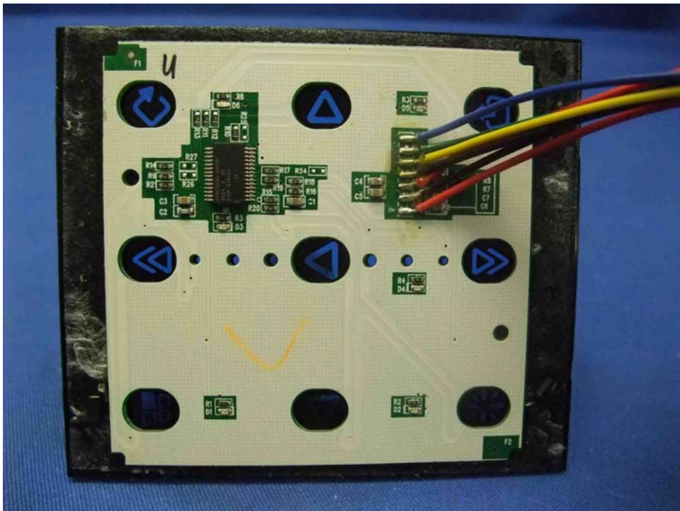
WiFi Internal Radio Player Keyboard front side (View 1)
