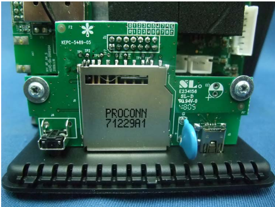
WiFi Internal Radio Player SD Card slot, USB Jack, and Power ON/OFF Switch PCB front side
