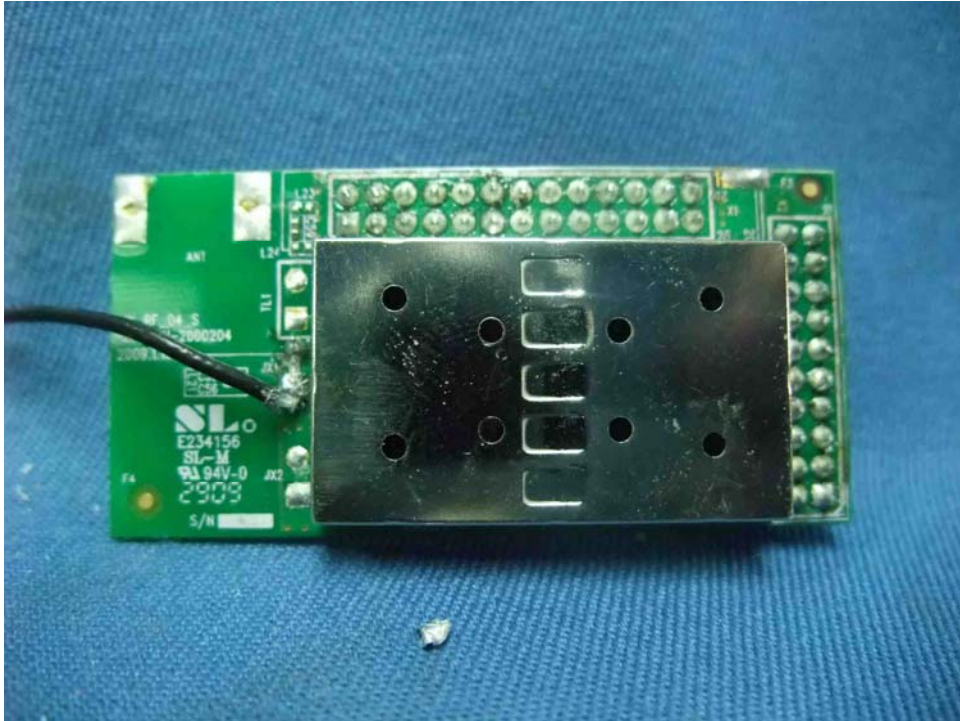
WiFi Internal Radio Player Antenna and RF module PCB front side (View 2)
