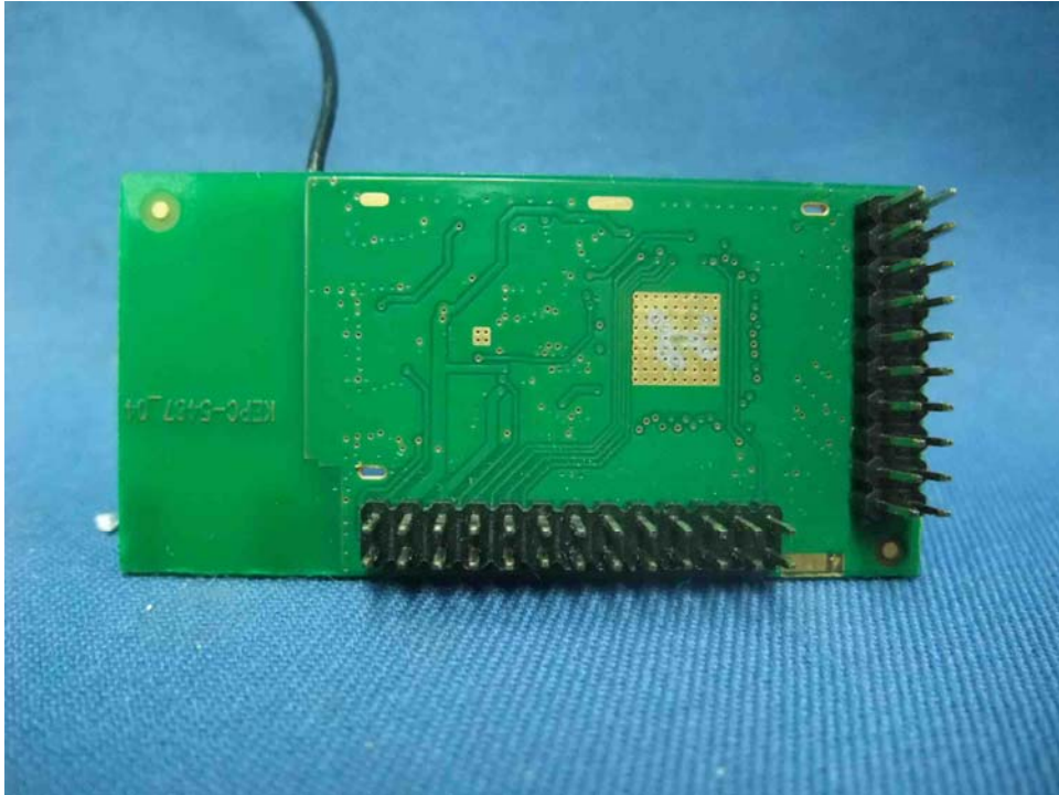
WiFi Internal Radio Player Antenna and RF module PCB rear side
