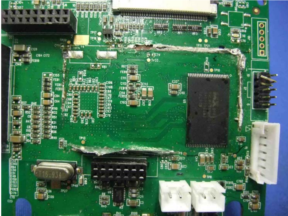
WiFi Internal Radio Player Main PCB rear side (View 3)
