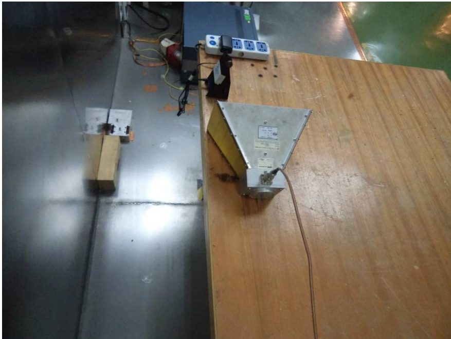
Conducted Emissions - Side View (Powered by adapter 1)
