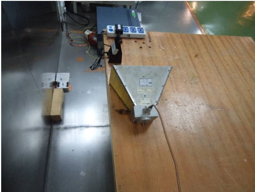
Conducted Emissions - Side View (Powered by adapter 2)
