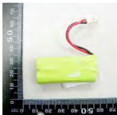
Figure 2. Battery(Ni-MH 3.6V 600mAh )
