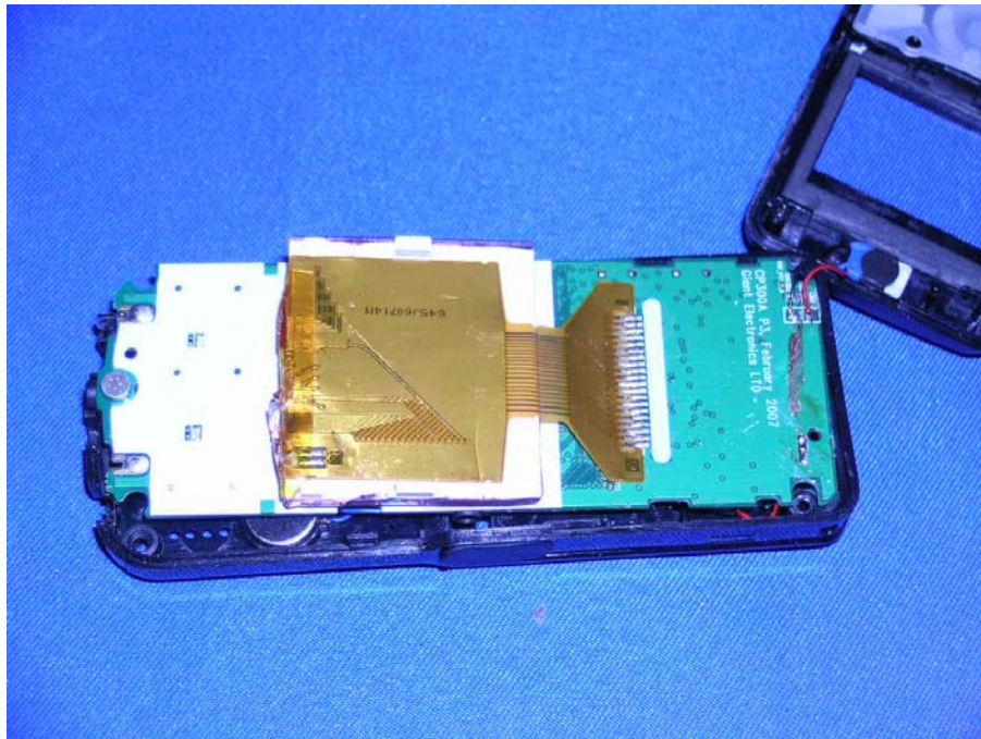
Wifi Phone Main PCB solder side (View 2)
