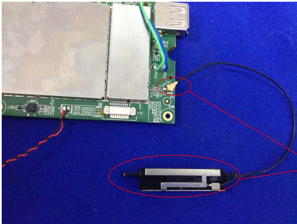
WIFI/BT ANTENNA
