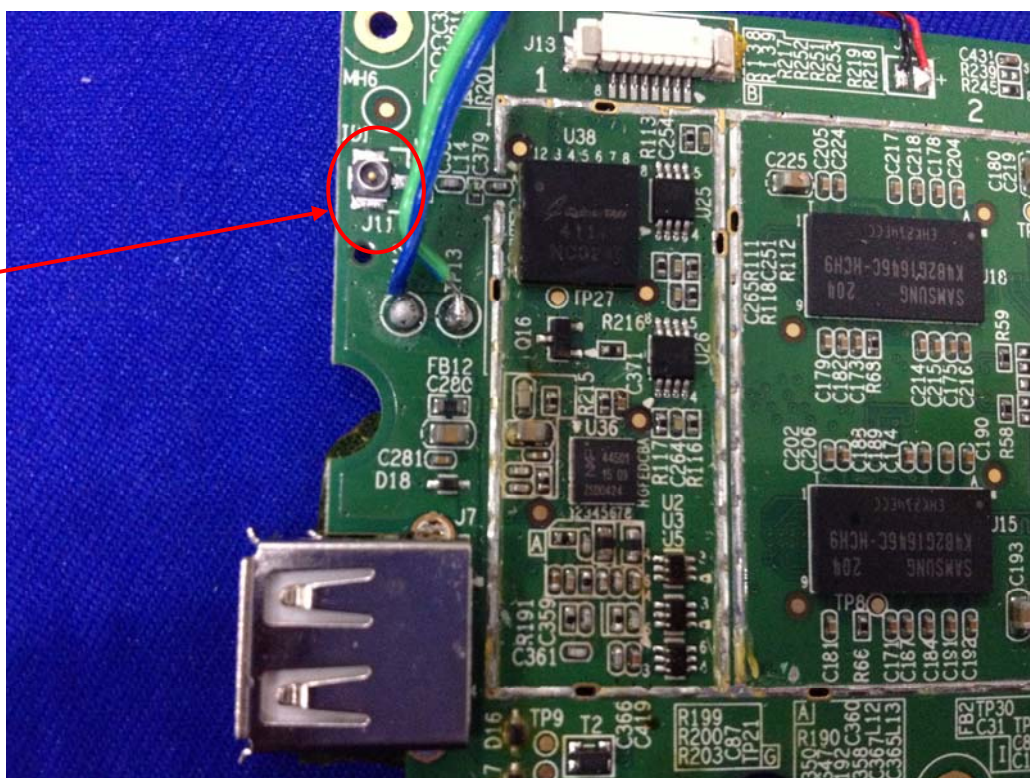
J11, WiFi/BT ANT
