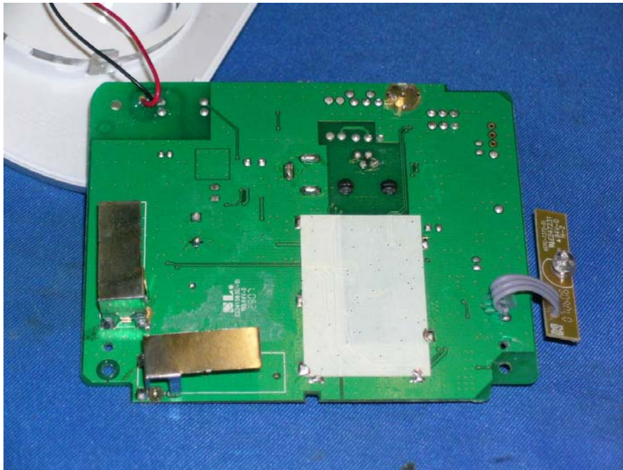
Base Unit Main PCB solder side (View 2)
