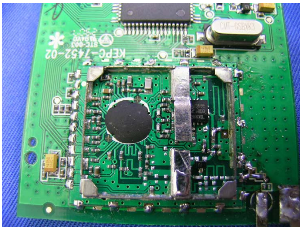
Parent Unit Oscillator PCB comp side (View 1)
