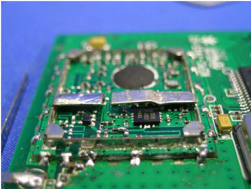
Parent Unit Oscillator PCB comp side (View 3)
