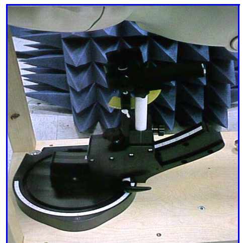
Figure 7. Device Holder
