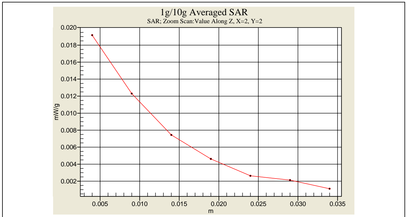
Face SAR Measurement _ Flat CH2
