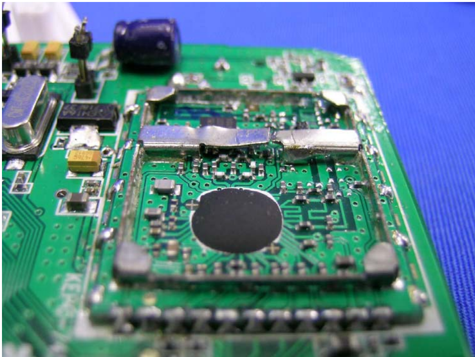
Baby Unit Oscillator PCB comp side (View 2)
