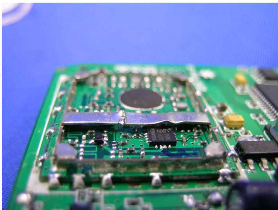
Baby Unit Oscillator PCB comp side (View 3)
