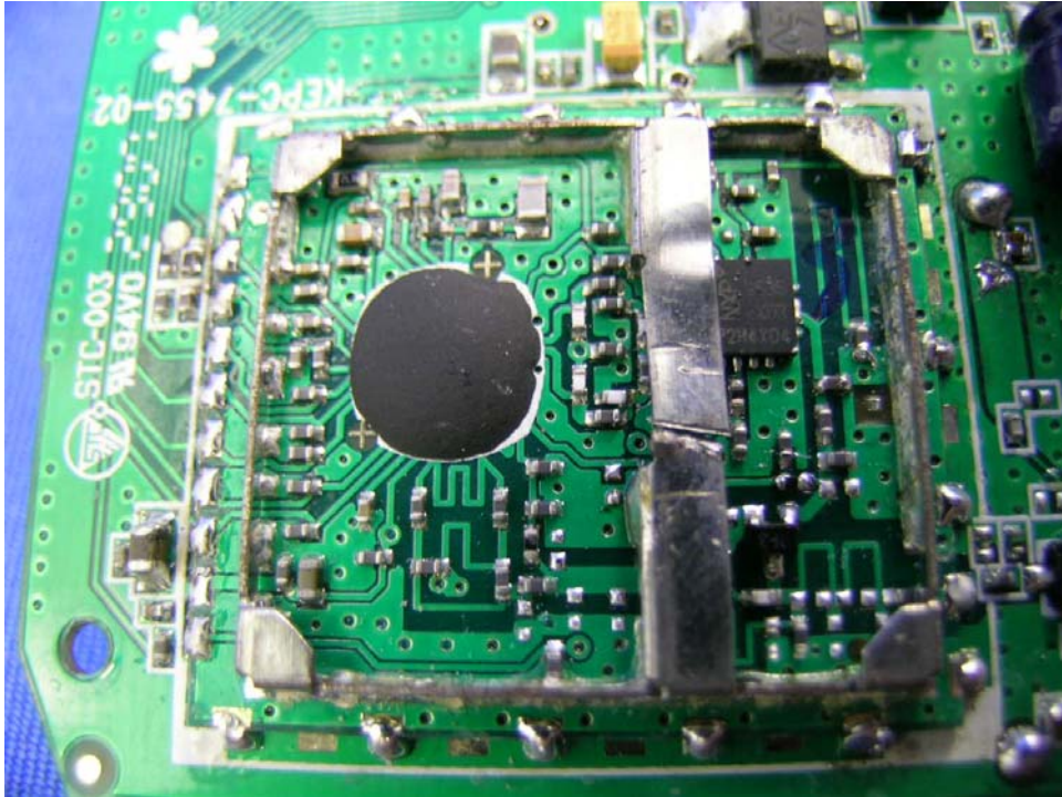
Baby Unit Oscillator PCB comp side (View 1)
