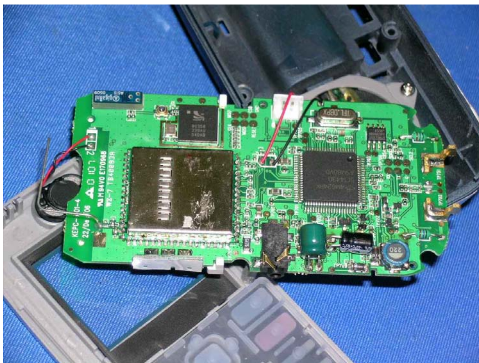
Bluetooth Main PCB comp side (View 1)
