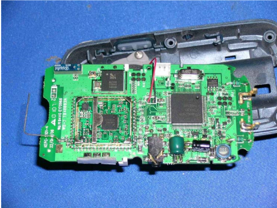
Bluetooth Main PCB comp side (View 2)
