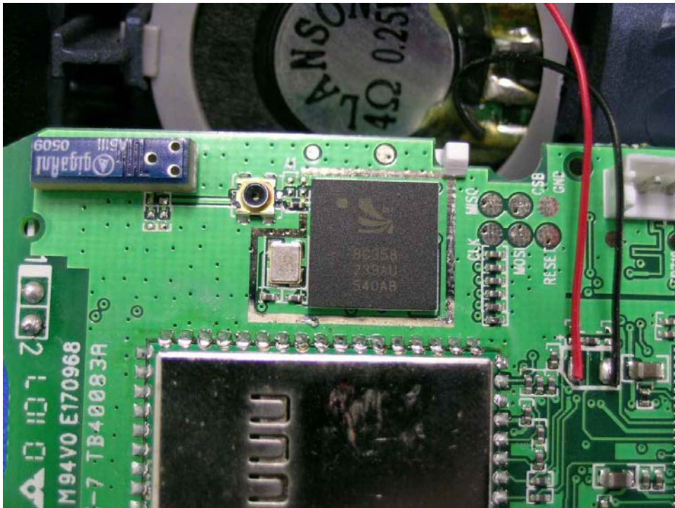
Bluetooth Oscillator PCB comp side
