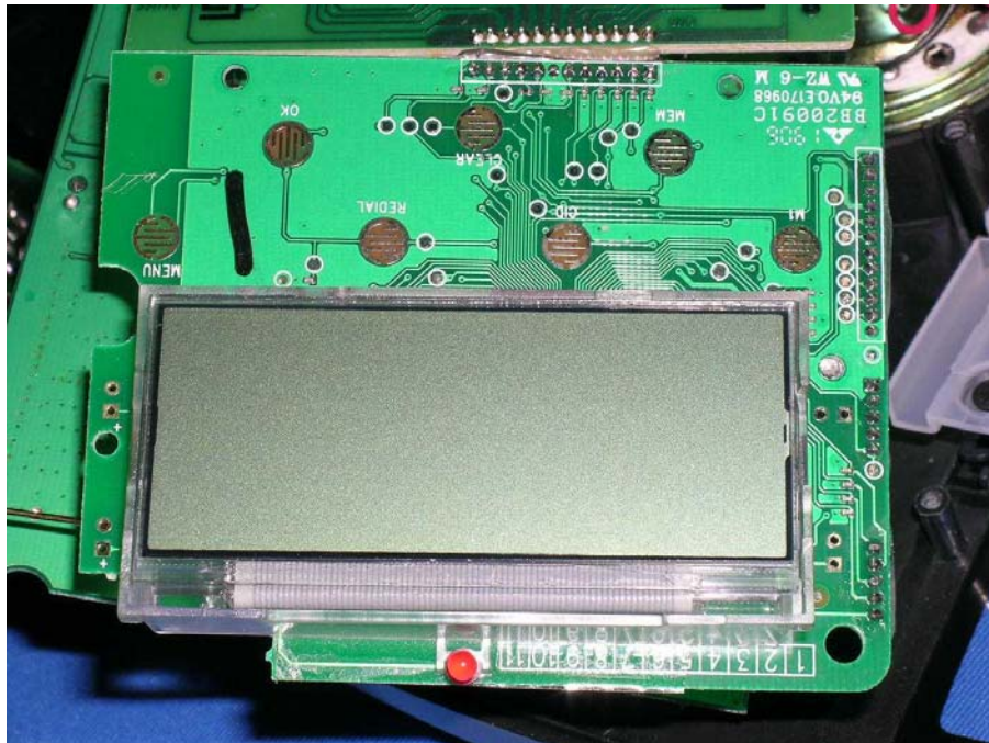
Base Unit Display front side (View 1)
