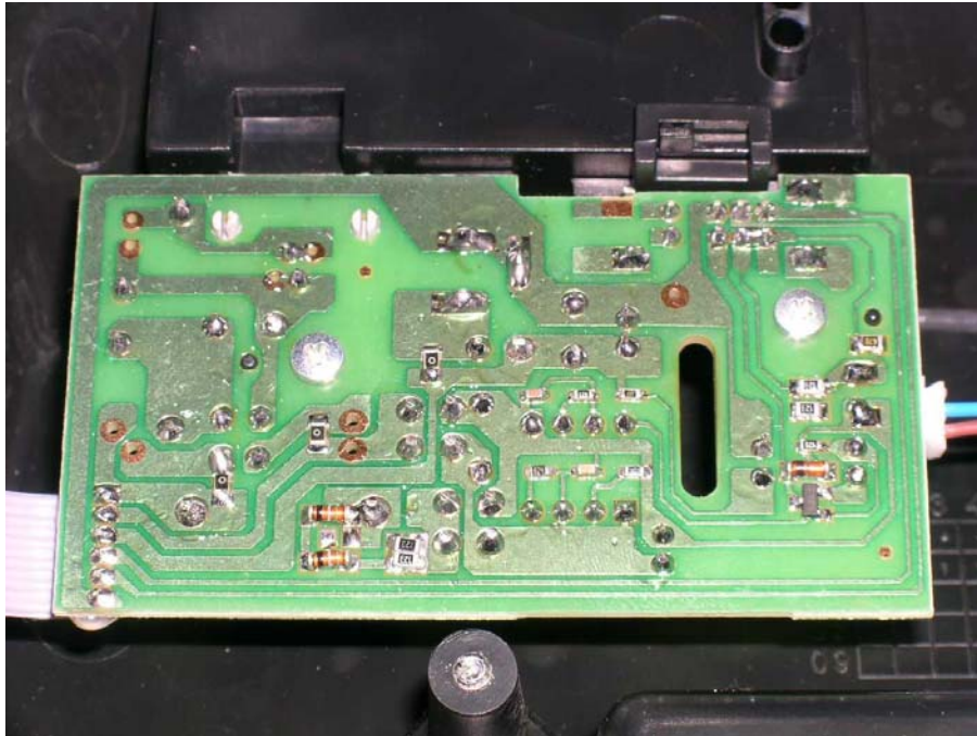
Base Unit DC Supply PCB solder side
