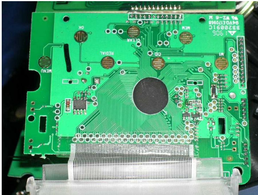
Base Unit Display front side (View 2)
