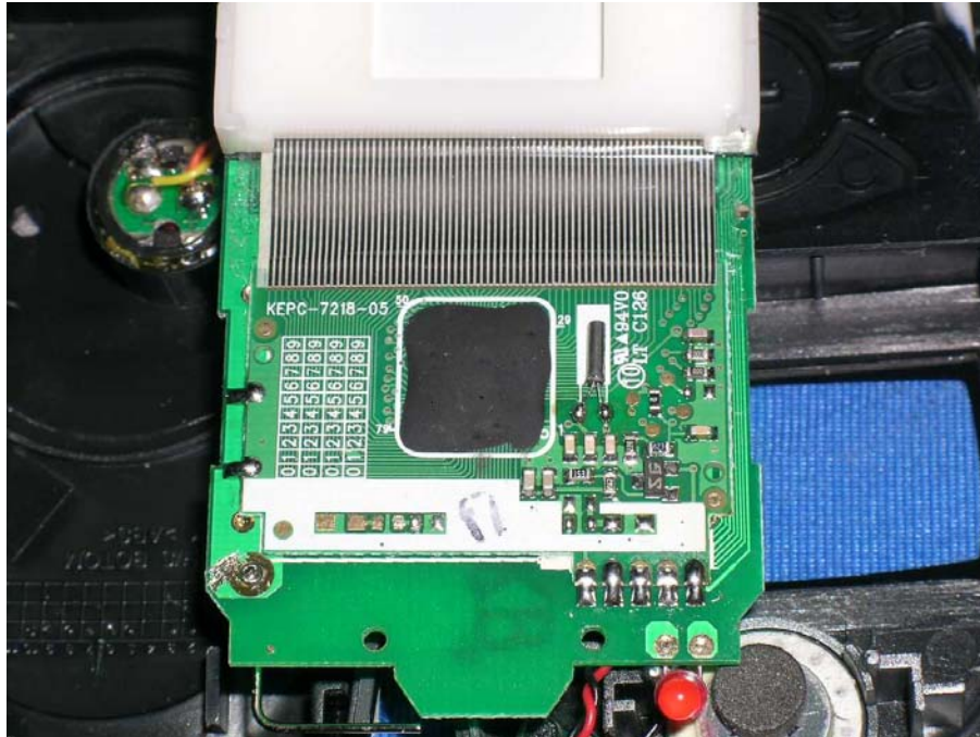
Handset Main PCB display side (View 3)
