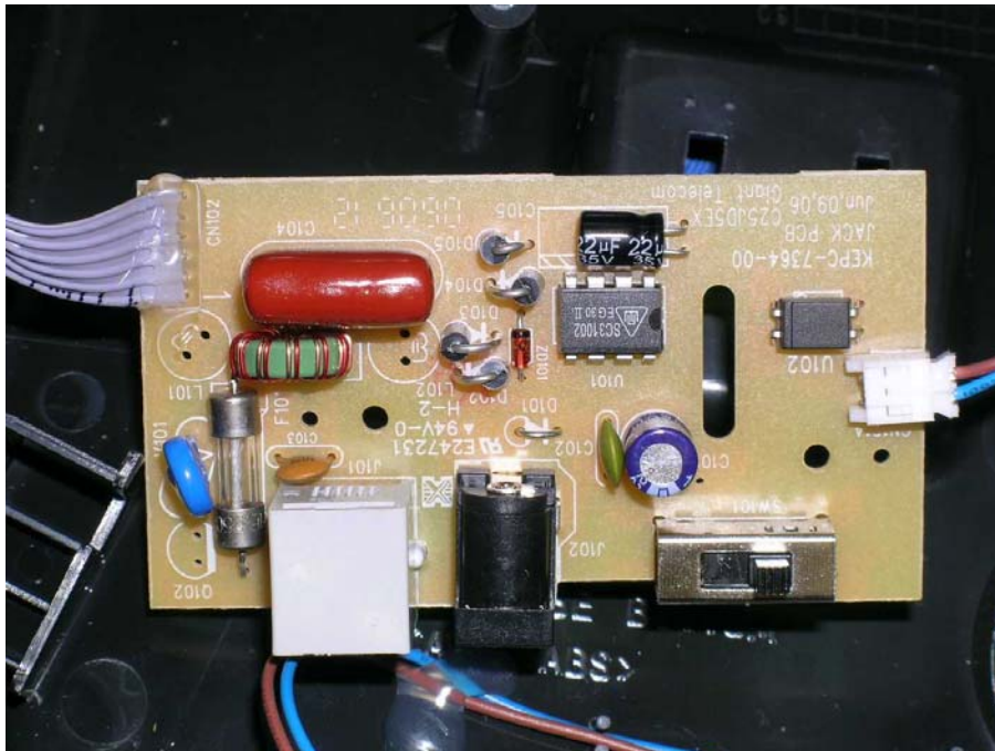
Base Unit DC Supply PCB comp side
