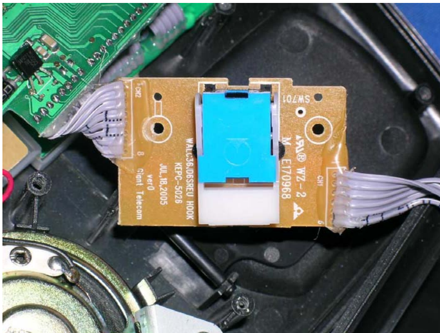
Base Unit On/Off Hook front side
