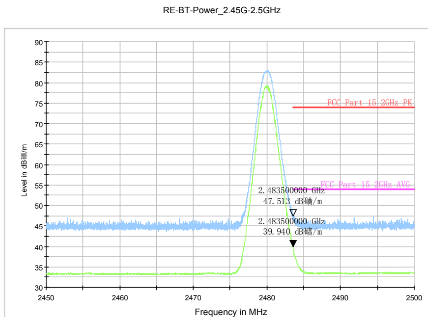
Fig.76. Radiated emission (Power): \pi/4 DQPSK, high channel
