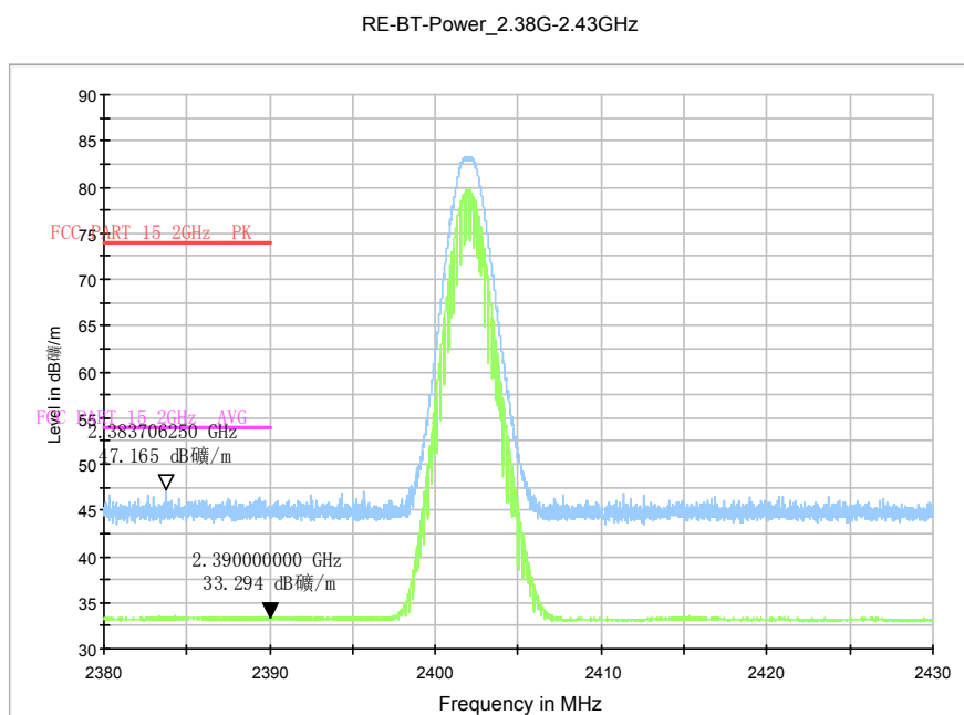
Fig.75. Radiated emission (Power): \pi/4 DQPSK, low channel
