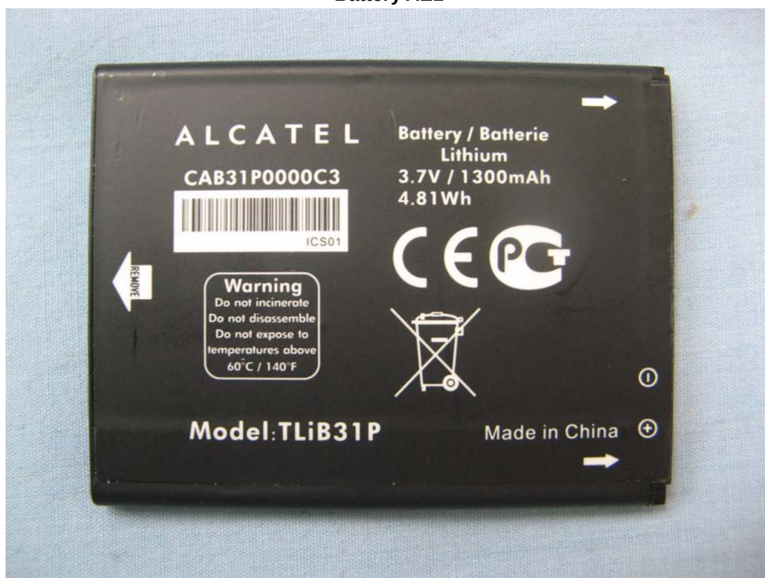
Battery AE2
