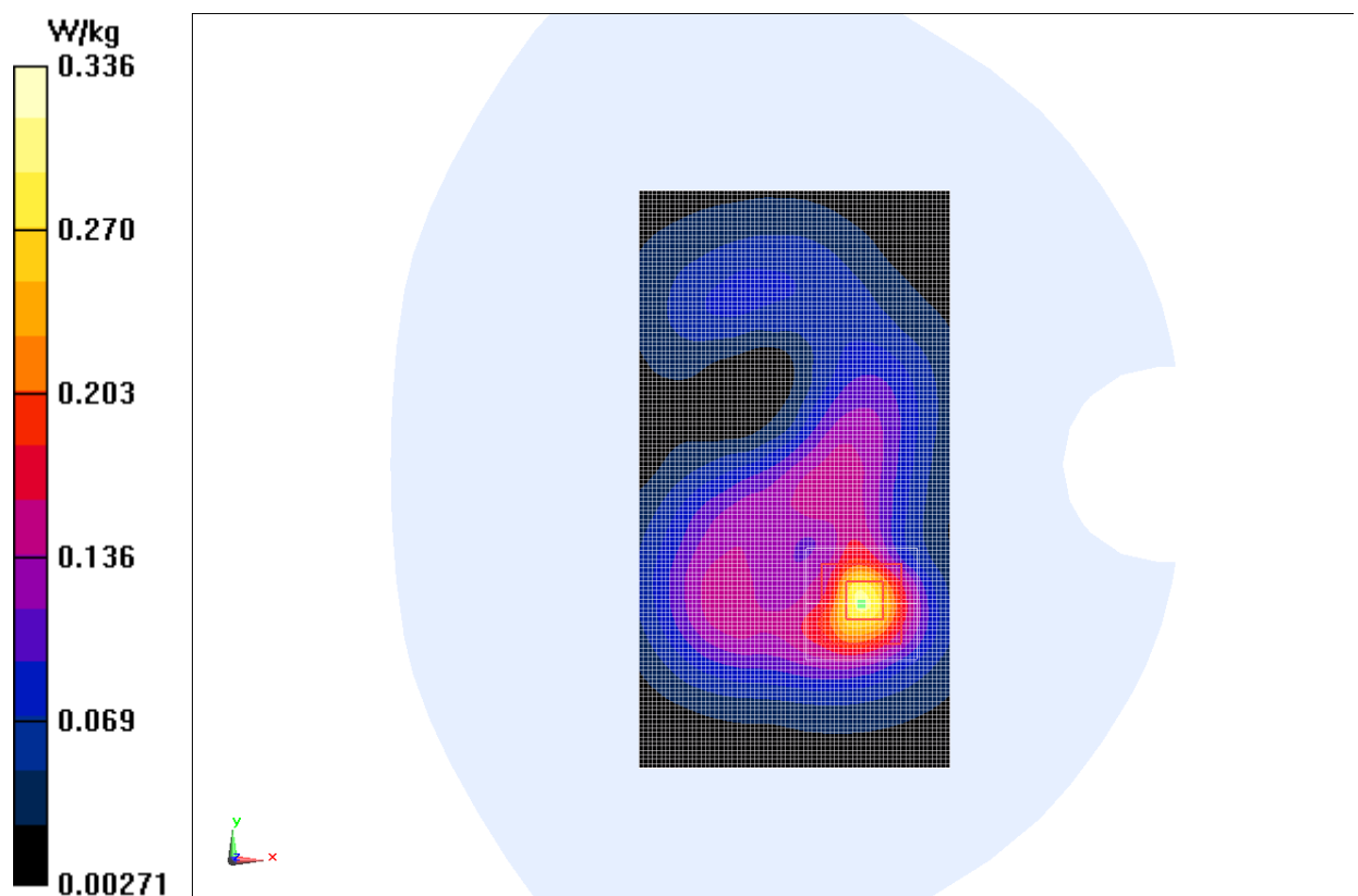
Fig.10 2450 MHz CH6
