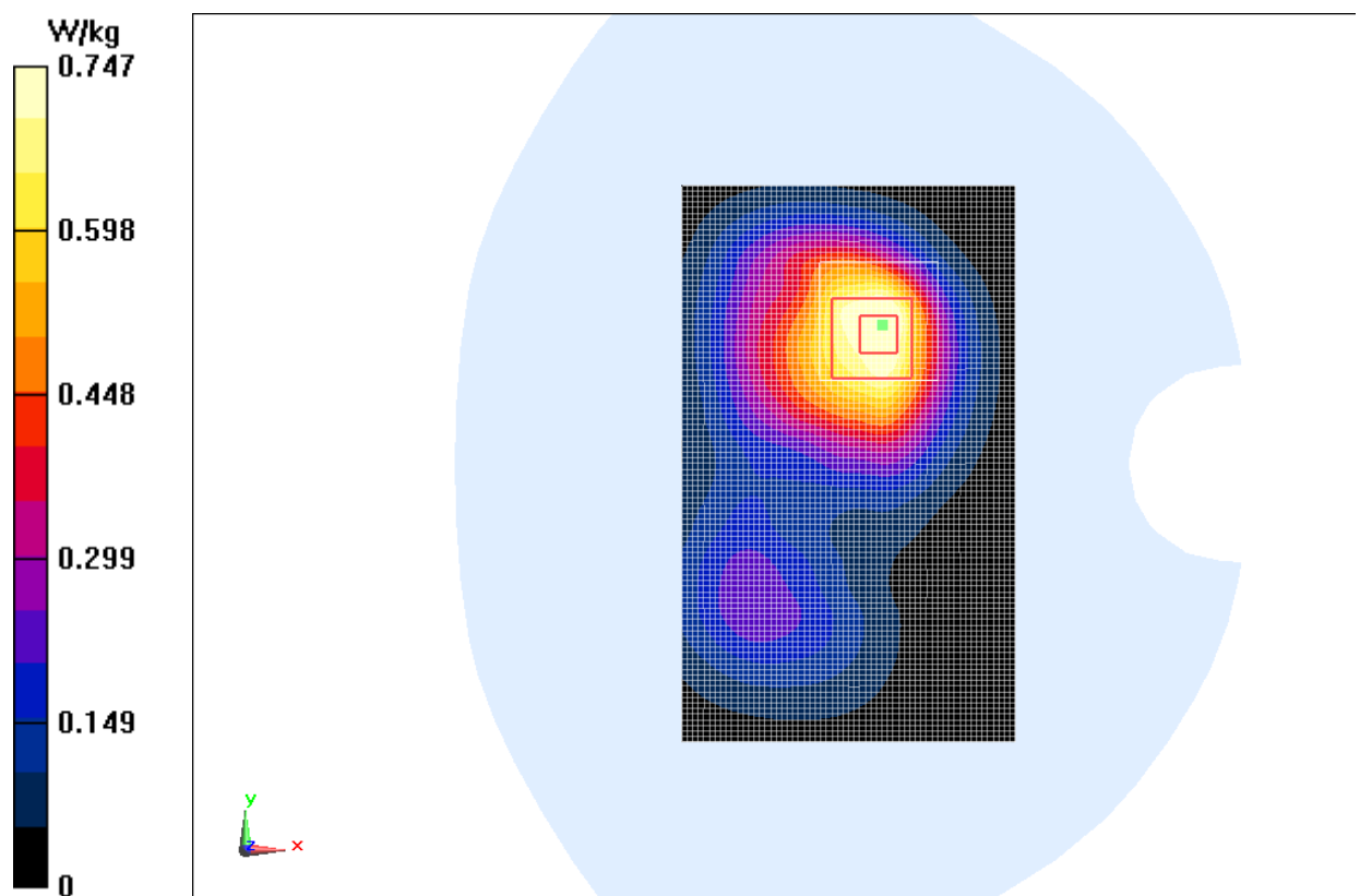
Fig.4 1900 MHz CH512
