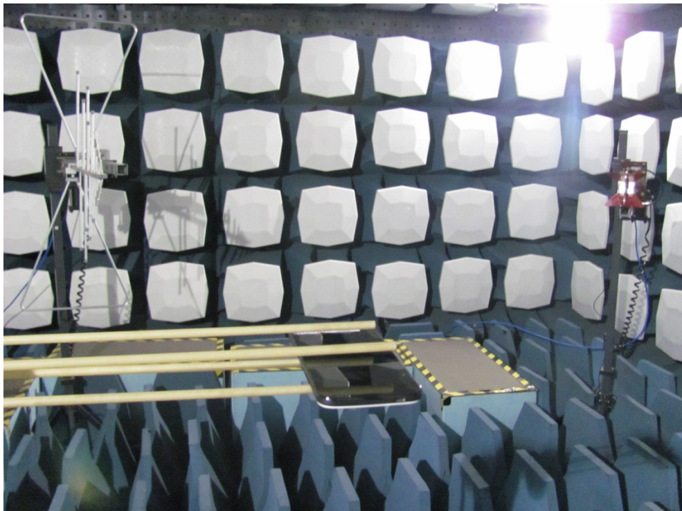
Pic F-1 Radiated Spurious Emission Test Layout
