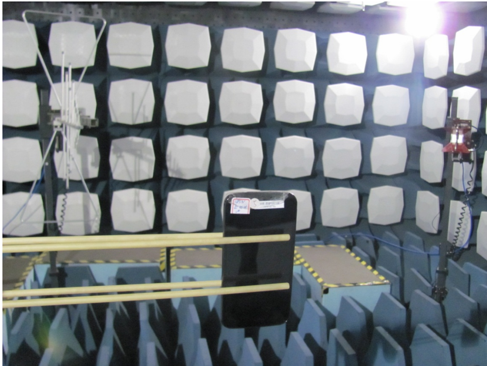
Pic F-2 Radiated Spurious Emission Test Layout
