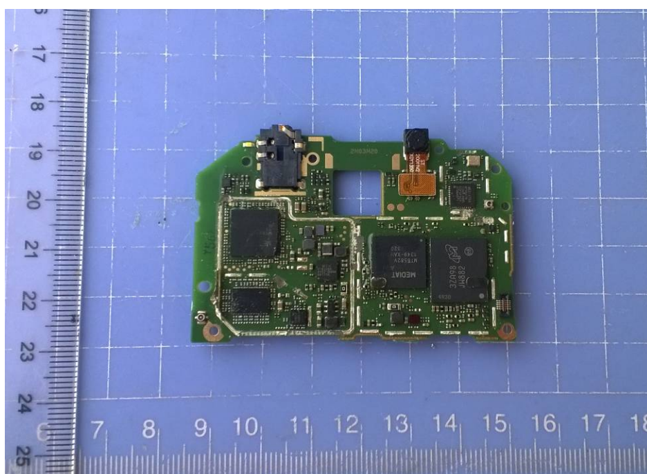
Pic A-8 Mobile phone Disassembly
