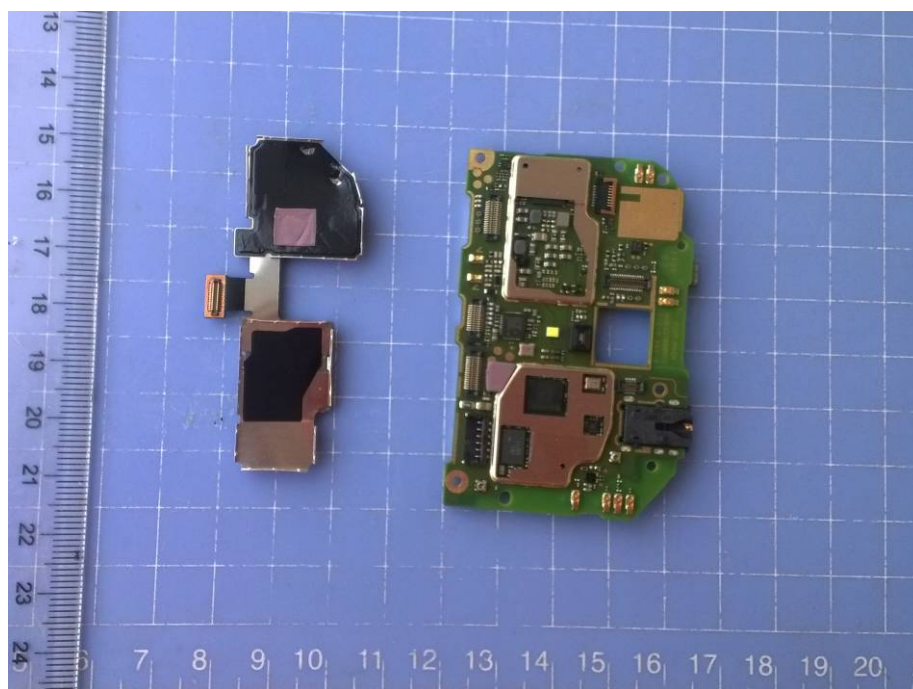
Pic A-7 Mobile phone Disassembly
