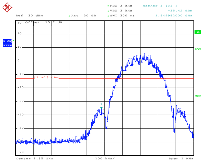
Lower Band Edge Plot on Channel 512 (1850.2 MHz)
