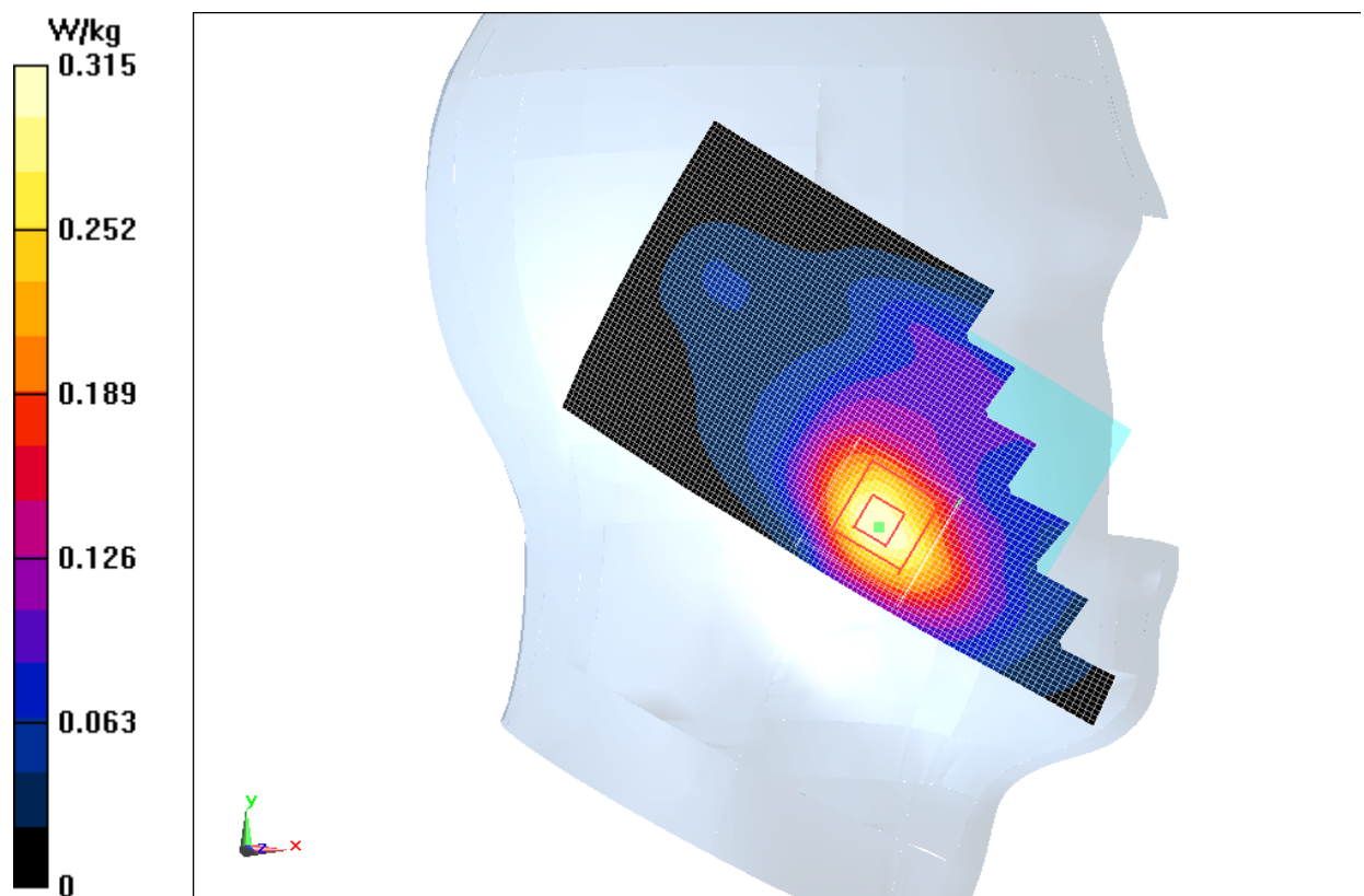
Fig.3 1900 MHz CH661
