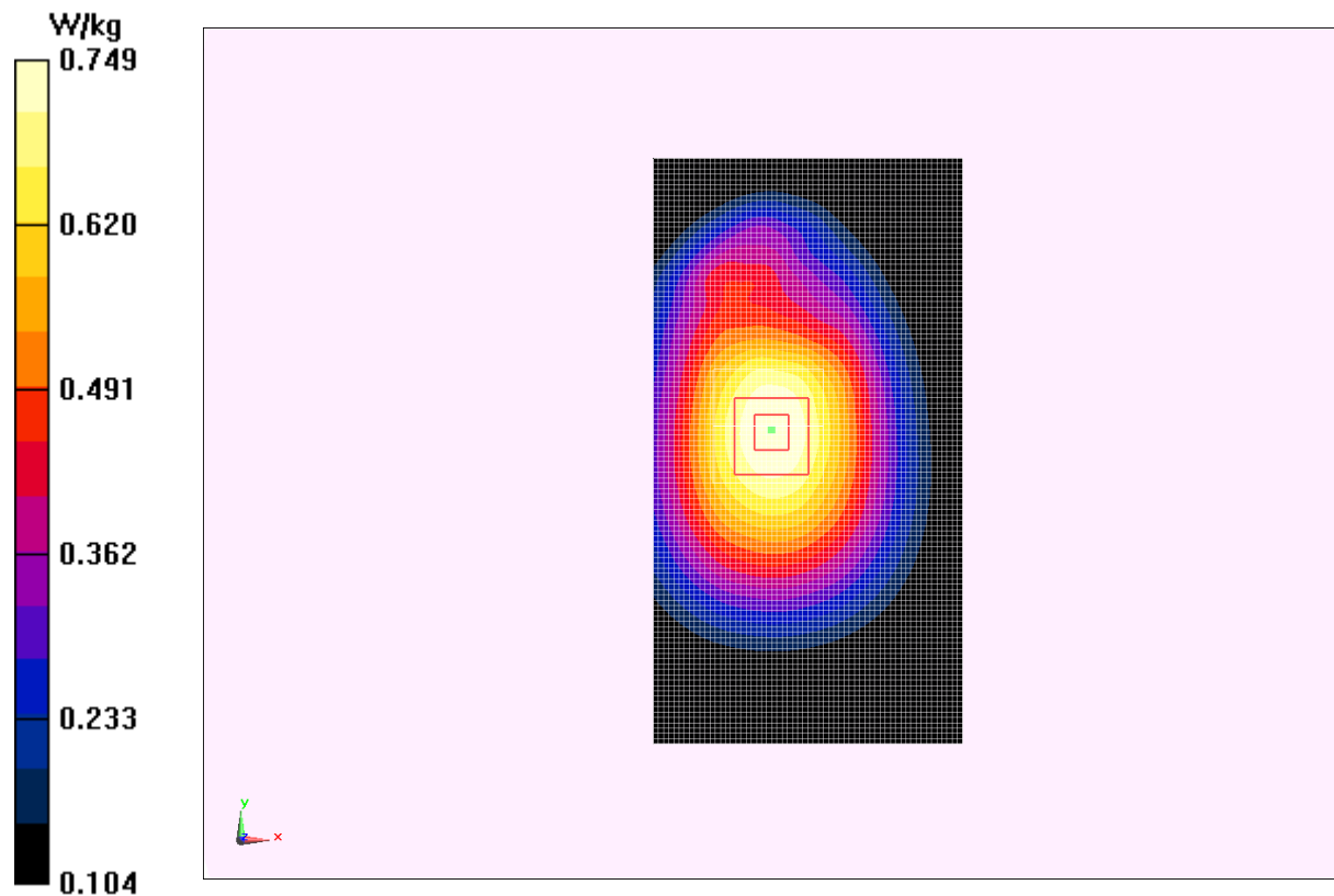
Fig.6 WCDMA 850 CH4233
