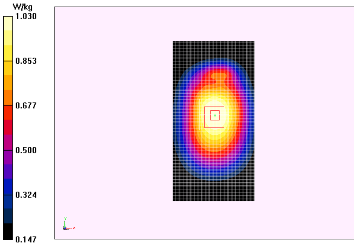
Fig.2 850 MHz CH251
