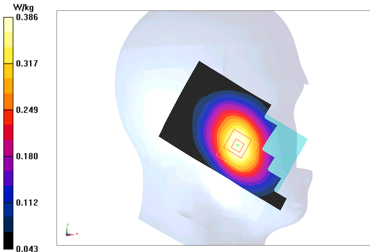
Fig.5 WCDMA 850 CH4233
