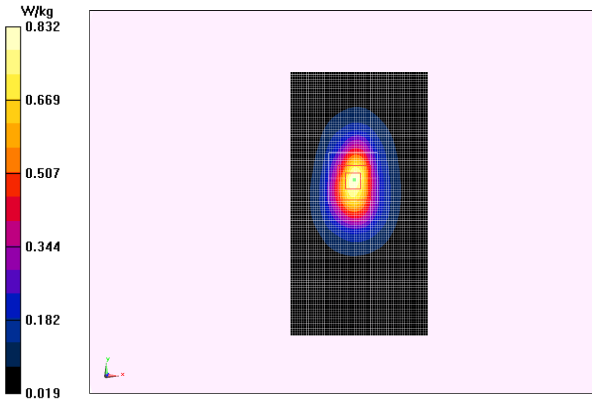
Fig.4 1900 MHz CH810
