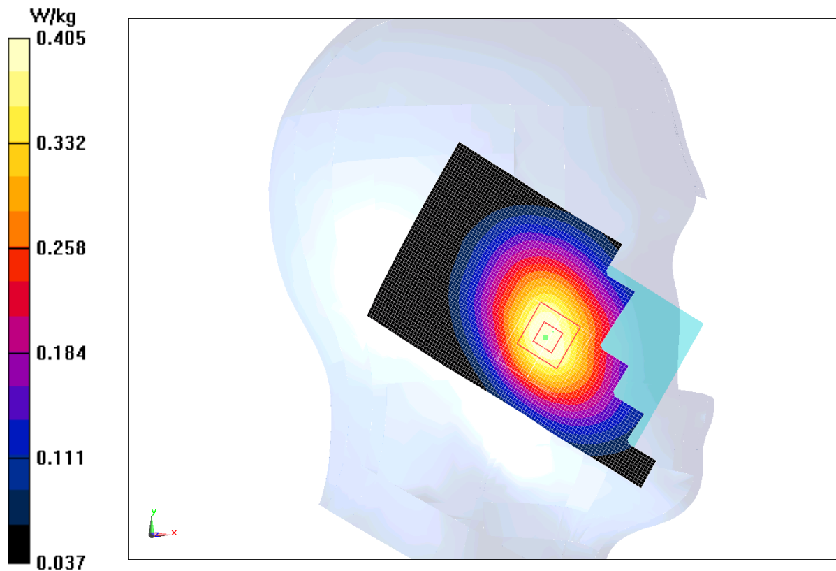
Fig.1 850MHz CH190
