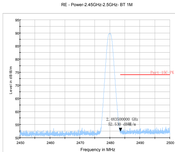
Fig.33. Radiated emission (Power): GFSK high channel (VBW=10Hz)
