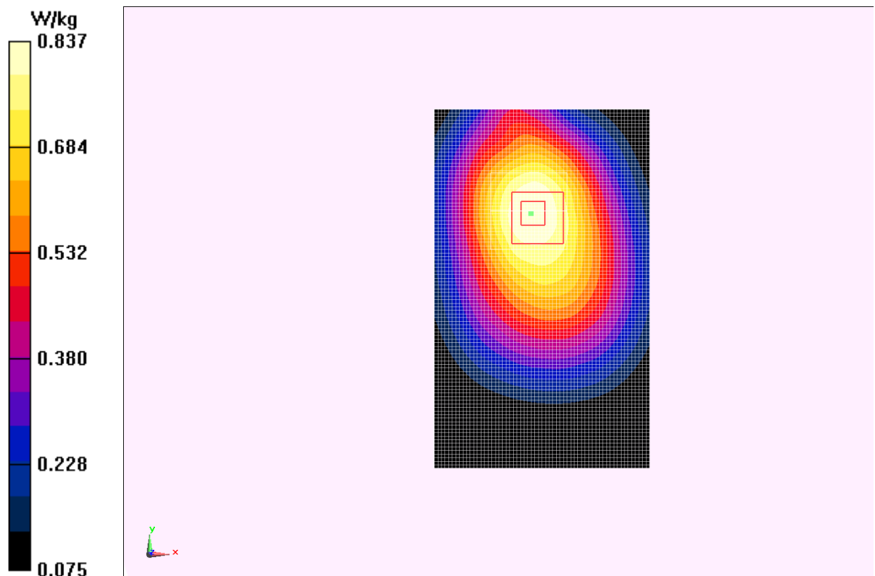
Fig.J.1 850 MHz CH128
