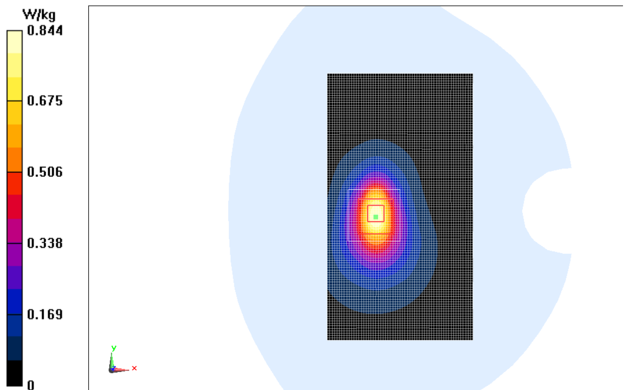
Fig.J.3 1900 MHz CH810
