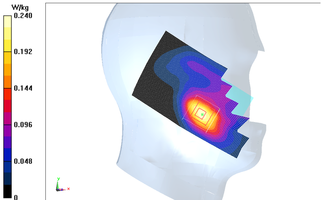
Fig.J.2 1900 MHz CH512
