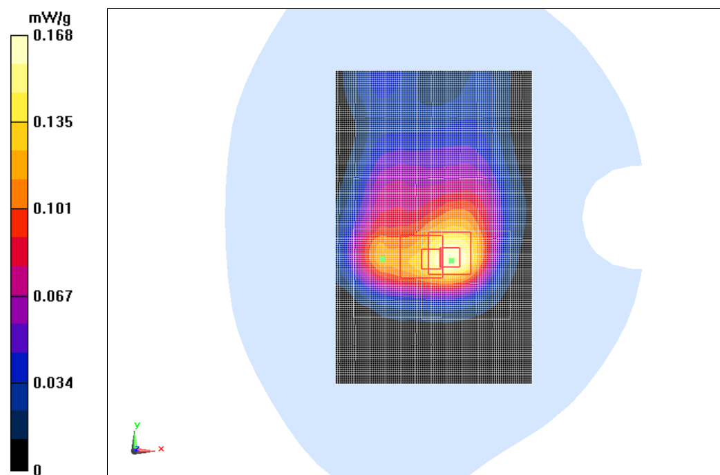
Fig.10 2450 MHz CH6
