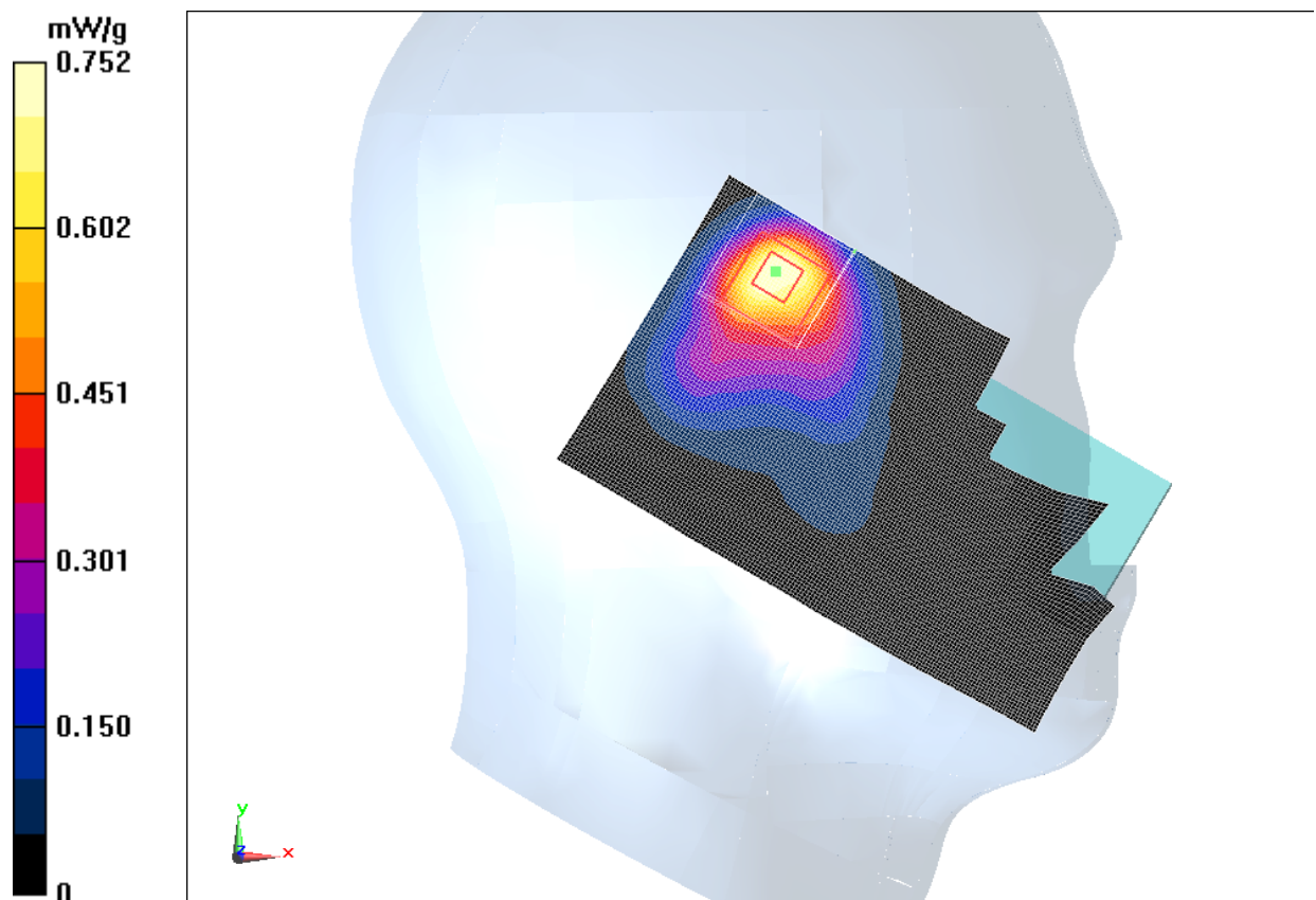
Fig.9 2450 MHz CH6
