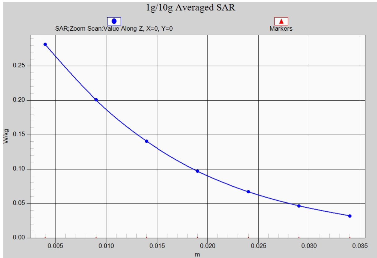
Fig. 8-1 Z-Scan at power reference point (WCDMA1700 CH1412)
