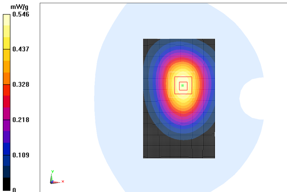
Fig. 19 850 MHz CH128
