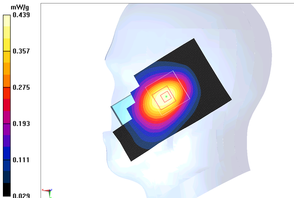
Fig.10 850 MHz CH251
