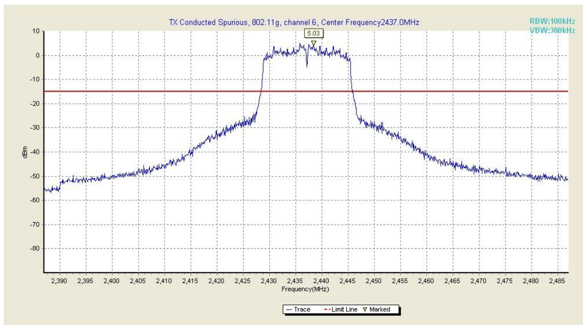
Fig. 33 Conducted Spurious Emission (802.11g, Ch6, Center Frequency)
