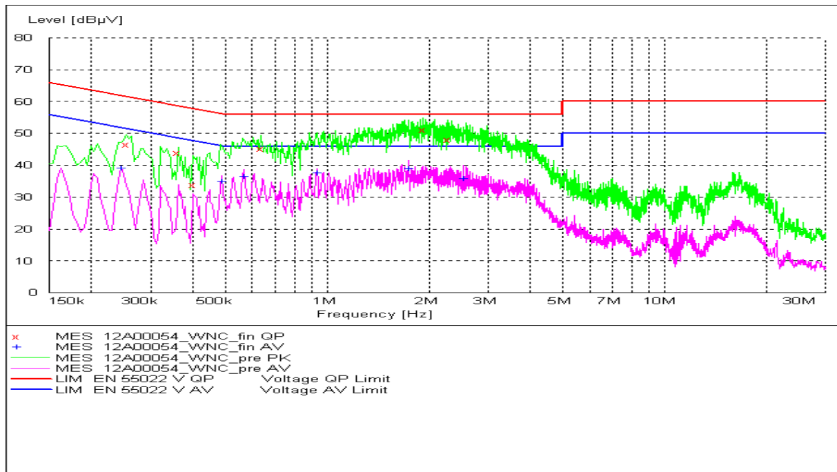
Fig. 79 AC Powerline Conducted Emission-802.11n mode
