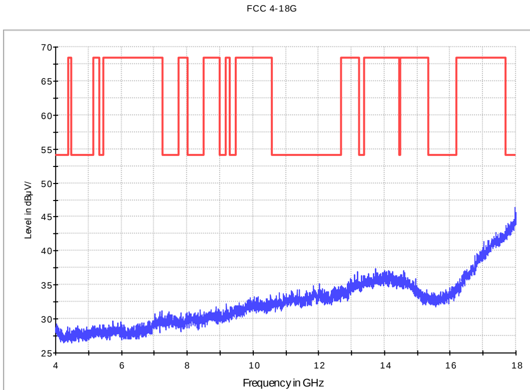
Fig. 75 Radiated Spurious Emission (802.11n-20MHz, Ch11, 4 GHz-18 GHz)
