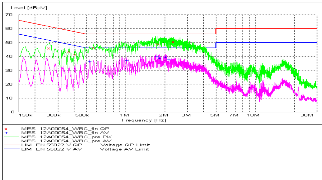
Fig. 77 AC Powerline Conducted Emission-802.11b mode
