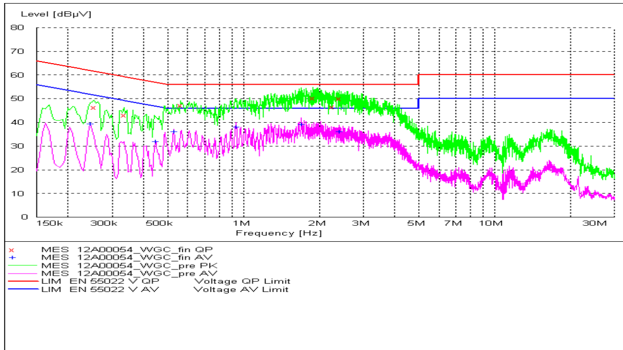
Fig. 78 AC Powerline Conducted Emission-802.11g mode
