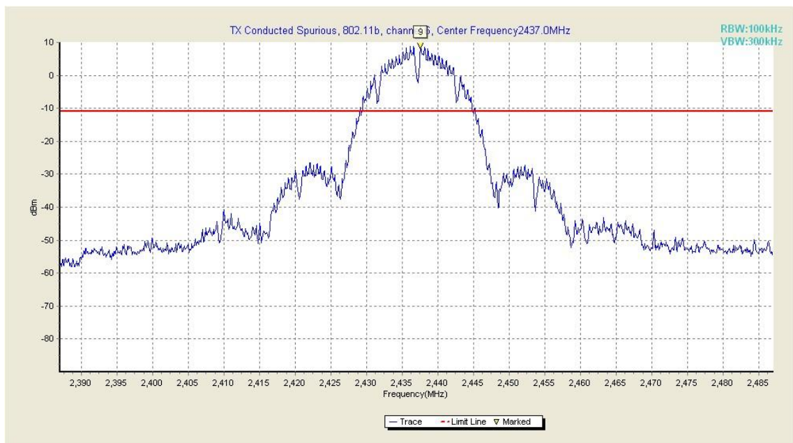
Fig. 27 Conducted Spurious Emission (802.11b, Ch6, Center Frequency)
