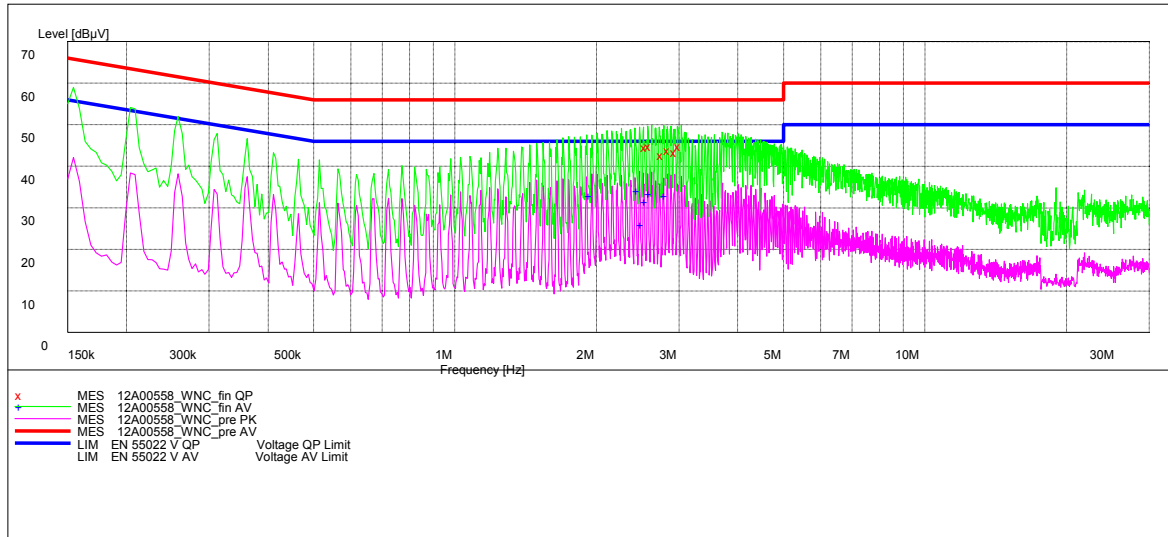
Fig. 77 AC Powerline Conducted Emission-802.11b
