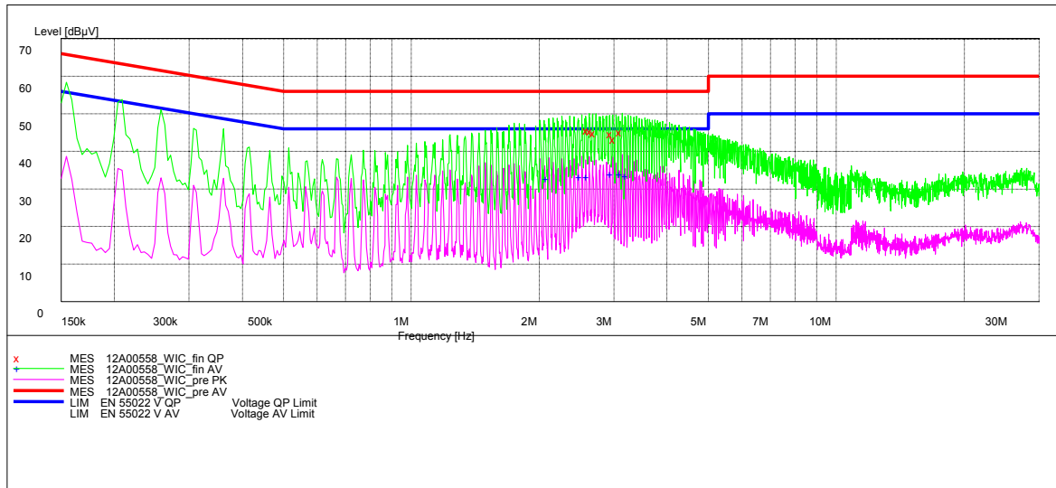
Fig. 78 AC Powerline Conducted Emission-802.11g
