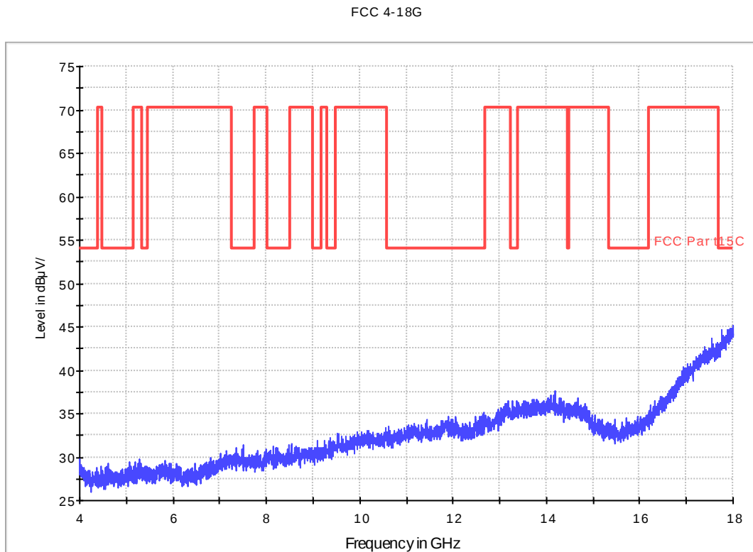
Fig. 49 Radiated Spurious Emission (802.11b, Ch6, 4 GHz-18 GHz)
