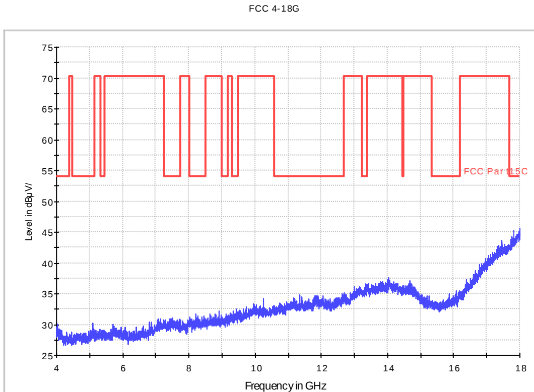
Fig. 71 Radiated Spurious Emission (802.11n-20MHz, Ch6, 4 GHz-18 GHz)
