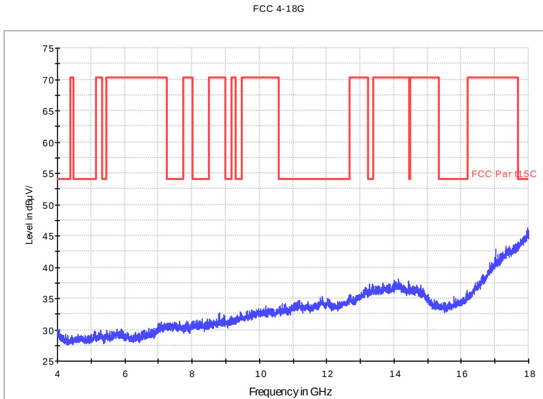
Fig. 57 Radiated Spurious Emission (802.11g, Ch1, 4 GHz-18 GHz)
