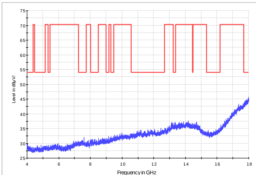
Fig. 64 Radiated Spurious Emission (802.11g, Ch11, 4 GHz-18 GHz)
