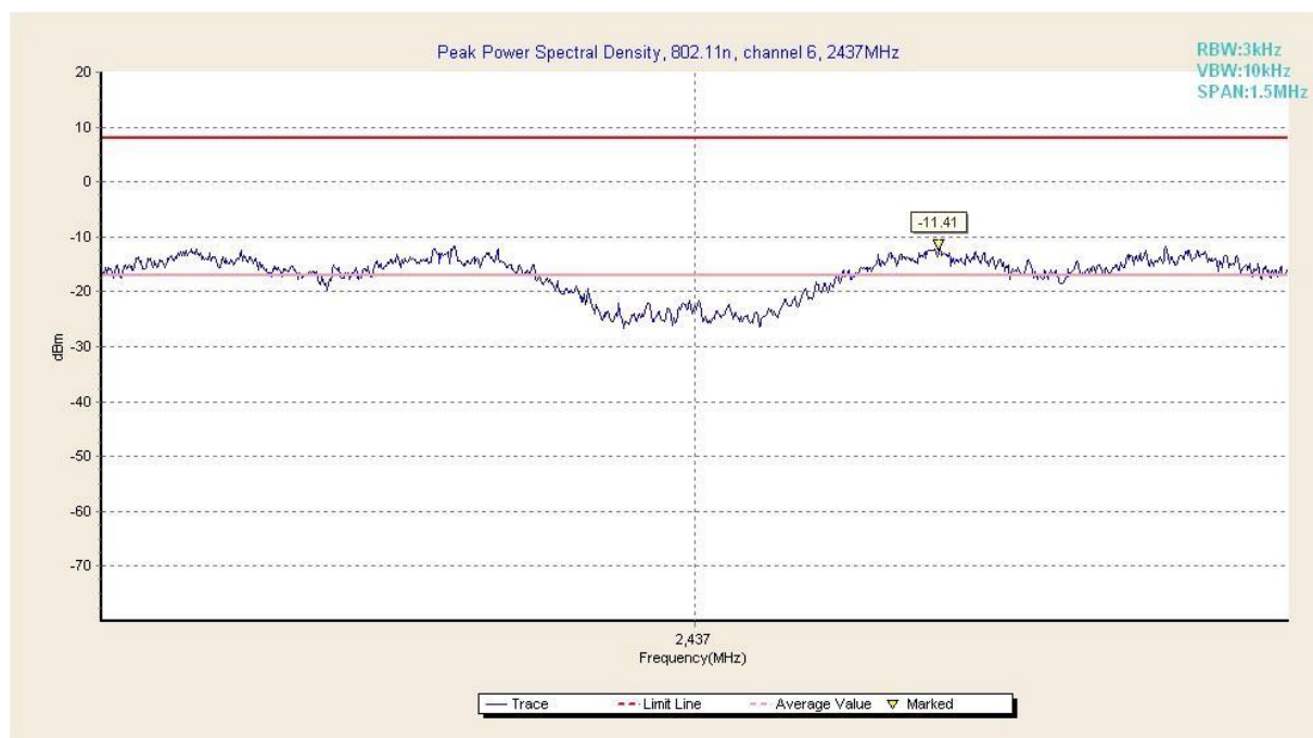
Fig. 8 Power Spectral Density (802.11n-20MHz, Ch 6)
