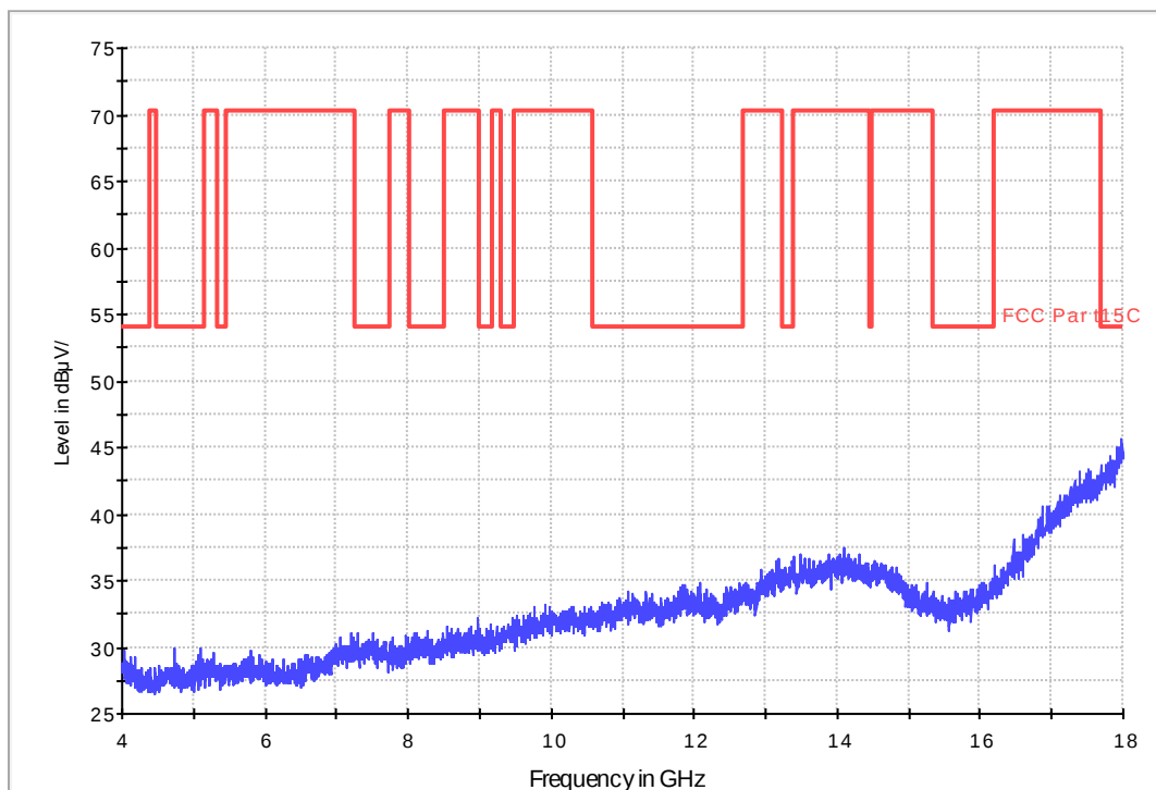
Fig. 60 Radiated Spurious Emission (802.11g, Ch6, 4 GHz-18 GHz)
