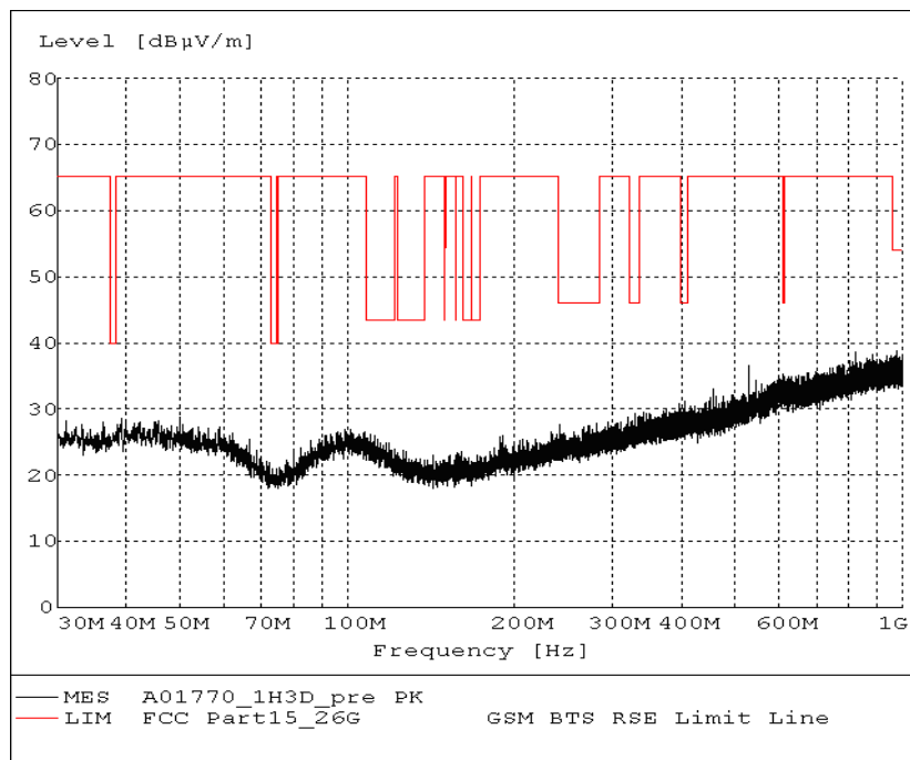
Fig.70. Radiated emission: 8DPSK, Channel 78, 30 MHz - 1 GHz
