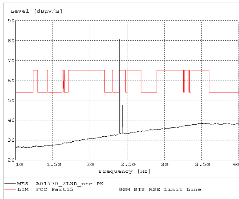
Fig.65. Radiated emission: 8DPSK, Channel 0, 1 GHz - 4 GHz
