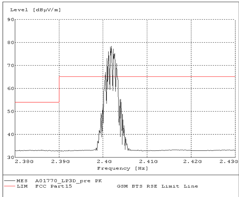
Fig.73. Radiated emission (Power): 8DPSK, low channel
