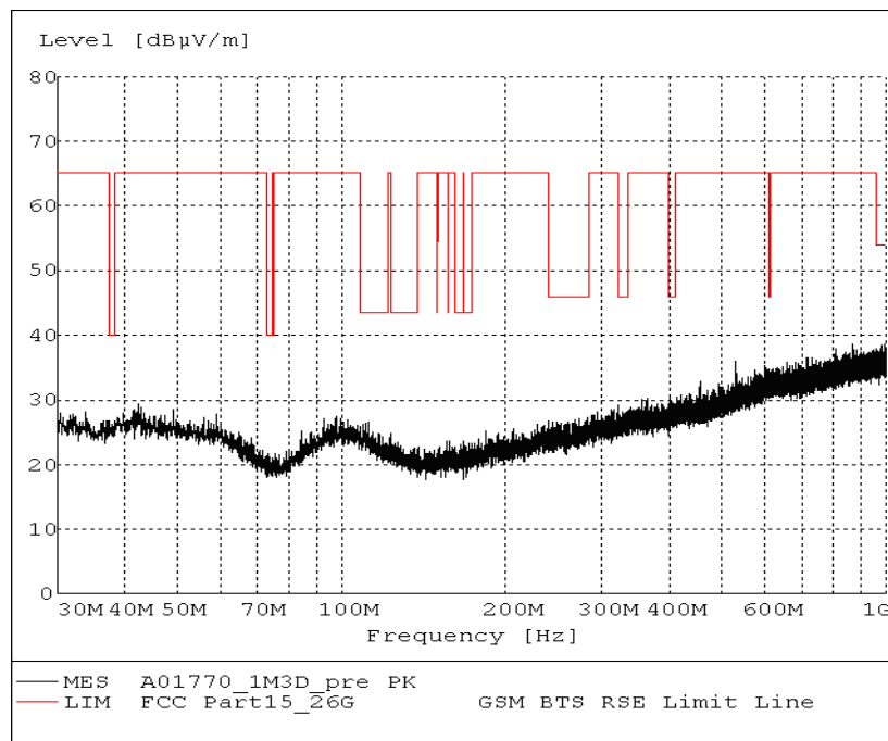
Fig.67. Radiated emission: 8DPSK, Channel 39, 30 MHz - 1 GHz
