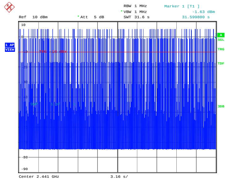
Fig.90 Time of occupancy (Dwell Time): Channel 39, Packet 3-DH3
