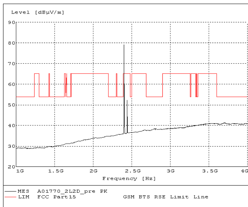
Fig.53. Radiated emission: \pi/4 DQPSK, Channel 0, 1 GHz - 4 GHz
