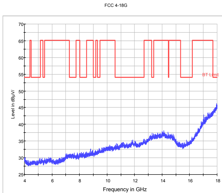
Fig.57. Radiated emission: \pi/4 DQPSK, Channel 39, 4 GHz - 18 GHz
