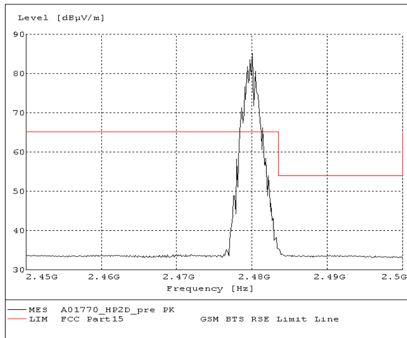
Fig.62. Radiated emission (Power): \pi/4 DQPSK, high channel
