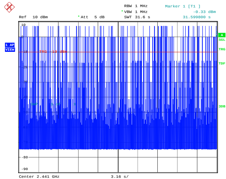
Fig.80 Time of occupancy (Dwell Time): Channel 39, Packet DH5
