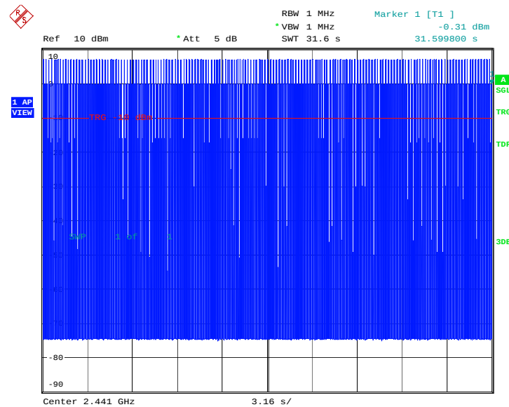
Fig.76 Time of occupancy (Dwell Time): Channel 39, Packet DH1
