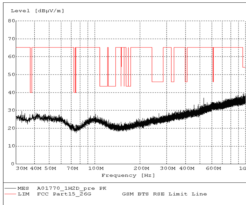
Fig.58. Radiated emission: \pi/4 DQPSK, Channel 78, 30 MHz - 1 GHz
