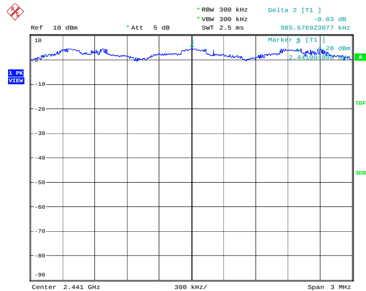
Fig.104 Carrier frequency separation measurement: \pi/4 DQPSK, Channel 39
