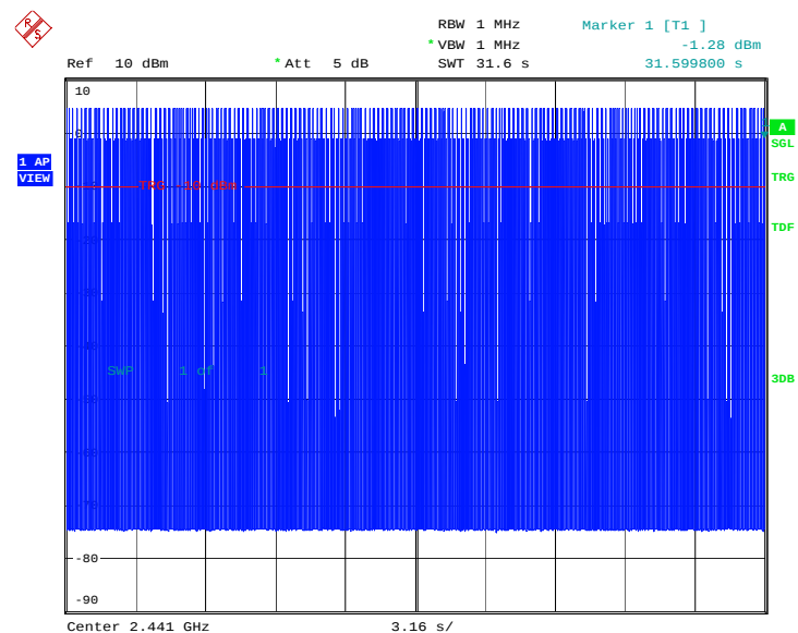
Fig.82 Time of occupancy (Dwell Time): Channel 39, Packet 2-DH1
