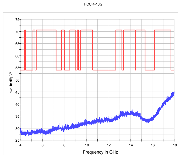
Fig.45. Radiated emission: GFSK, Channel 39, 4 GHz - 18 GHz
