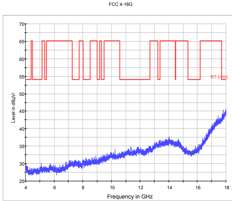
Fig.72. Radiated emission: 8DPSK, Channel 78, 4 GHz - 18 GHz
