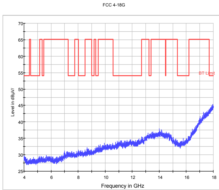
Fig.54. Radiated emission: \pi/4 DQPSK, Channel 0, 4 GHz - 18 GHz
