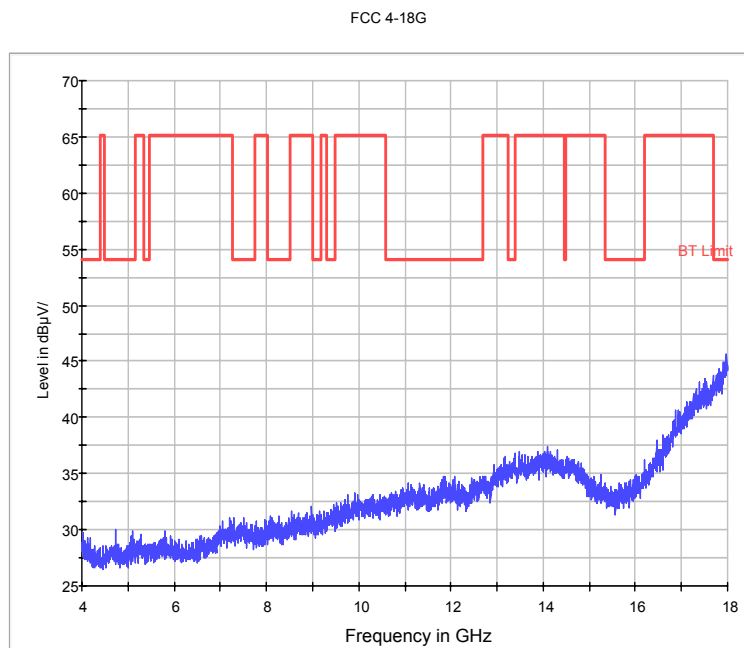
Fig.69. Radiated emission: 8DPSK, Channel 39, 4 GHz - 18 GHz
