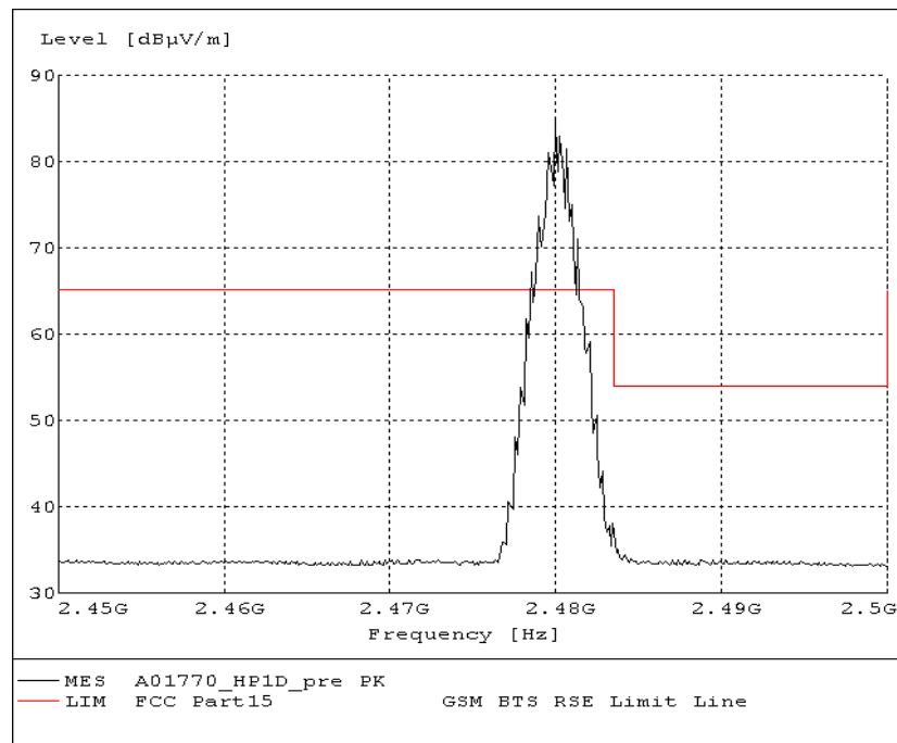
Fig.50. Radiated emission (Power) GFSK, high channel
