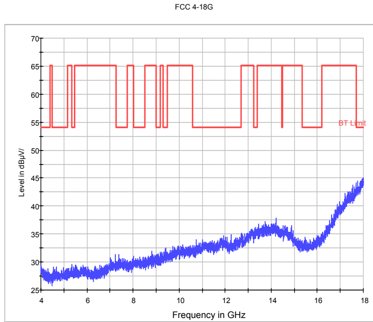
Fig.48. Radiated emission: GFSK, Channel 78, 4 GHz - 18 GHz
