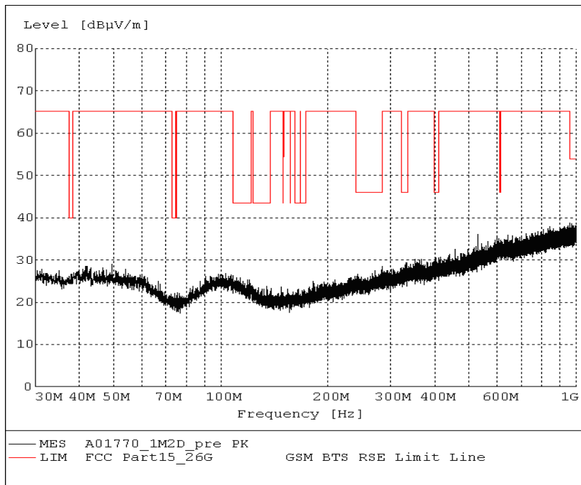
Fig.55. Radiated emission: \pi/4 DQPSK, Channel 39, 30 MHz - 1 GHz
