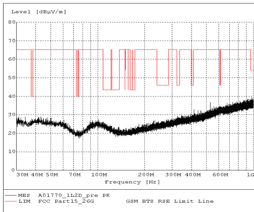
Fig.52. Radiated emission: \pi/4 DQPSK, Channel 0, 30 MHz - 1 GHz
