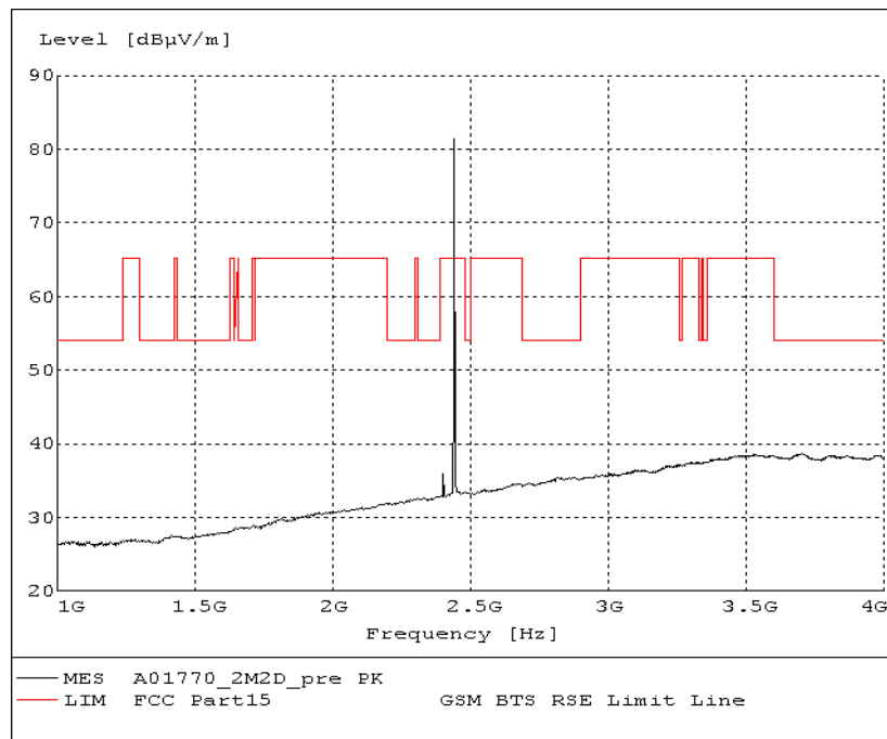
Fig.56. Radiated emission: \pi/4 DQPSK, Channel 39, 1 GHz - 4 GHz
