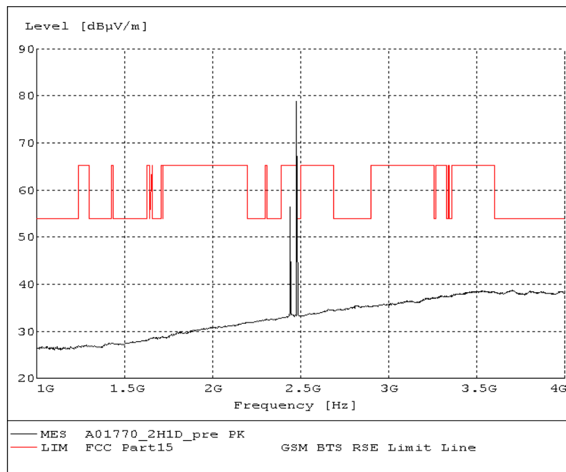
Fig.47. Fig.47 Radiated emission: GFSK, Channel 78, 1 GHz - 4 GHz
