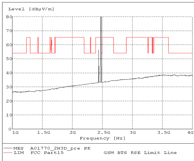
Fig.71. Radiated emission: 8DPSK, Channel 78, 1 GHz - 4 GHz
