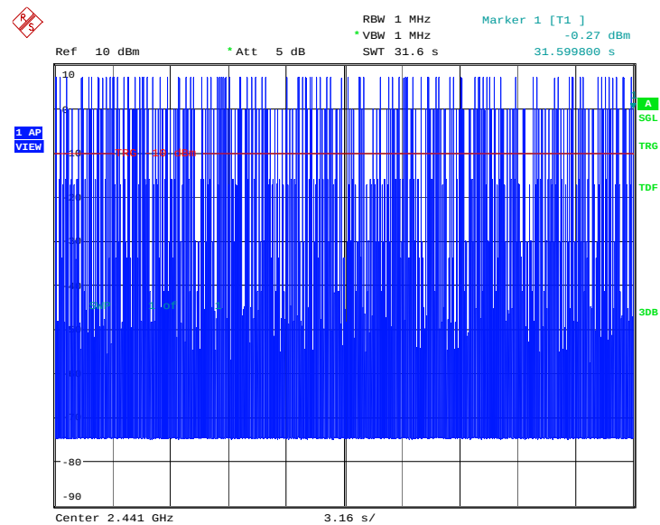
Fig.78 Time of occupancy (Dwell Time): Channel 39, Packet DH3
