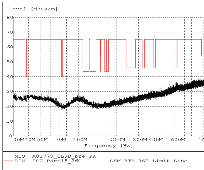
Fig.64. Radiated emission: 8DPSK, Channel 0, 30 MHz - 1 GHz
