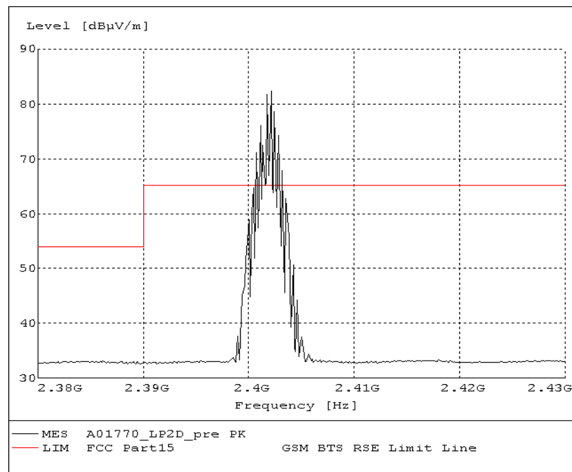
Fig.61. Radiated emission (Power): \pi/4 DQPSK, low channel
