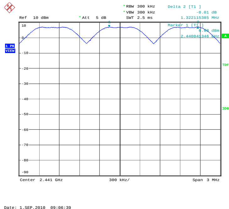
Fig.103 Carrier frequency separation measurement: GFSK, Channel 39
