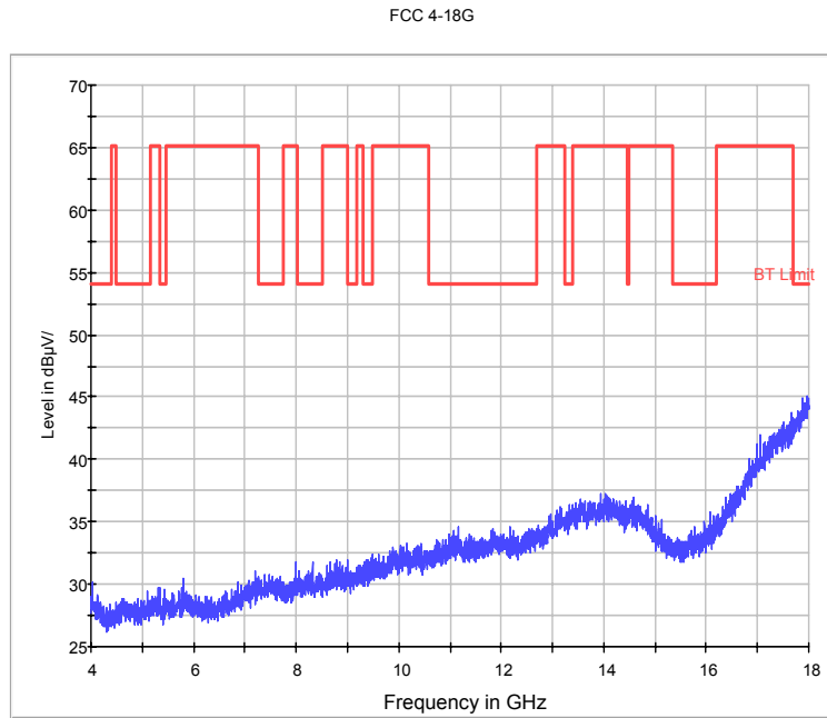
Fig.42. Radiated emission: GFSK, Channel 0, 4 GHz - 18 GHz
