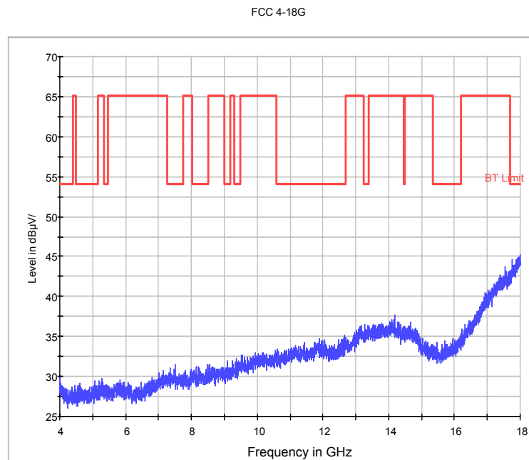
Fig.66. Radiated emission: 8DPSK, Channel 0, 4 GHz - 18 GHz
