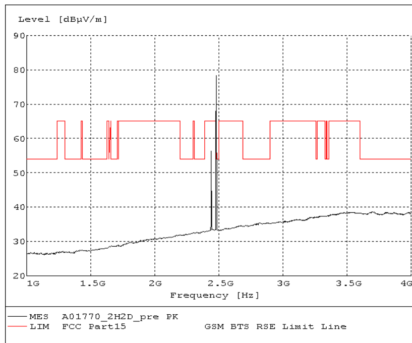
Fig.59. Radiated emission: \pi/4 DQPSK, Channel 78, 1 GHz - 4 GHz
