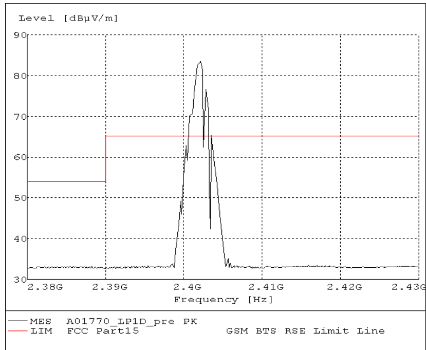
Fig.49. Radiated emission (Power): GFSK, low channel
