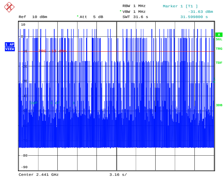
Fig.92 Time of occupancy (Dwell Time): Channel 39, Packet 3-DH5
