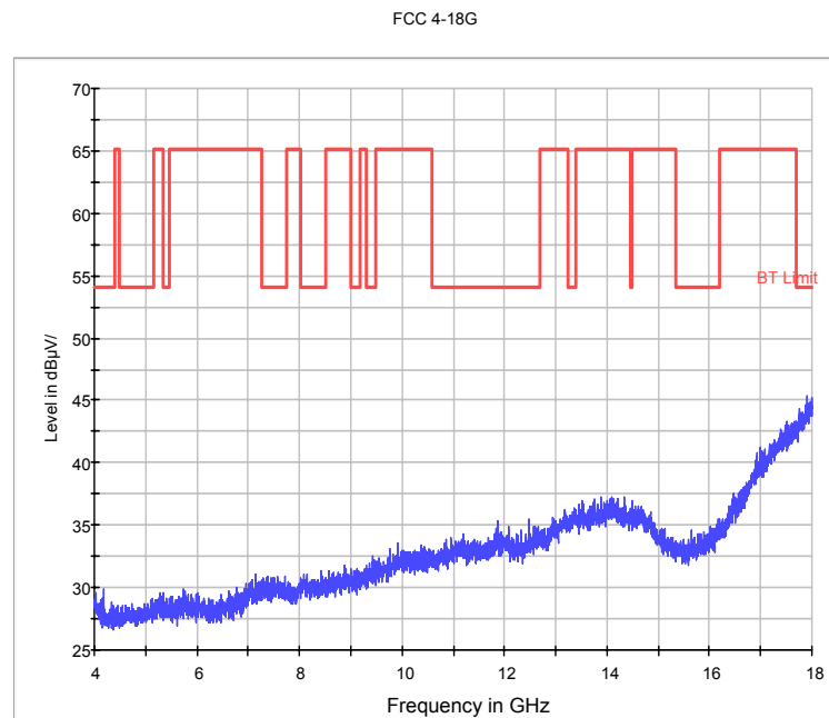
Fig.60. Radiated emission: \pi/4 DQPSK, Channel 78, 4 GHz - 18 GHz
