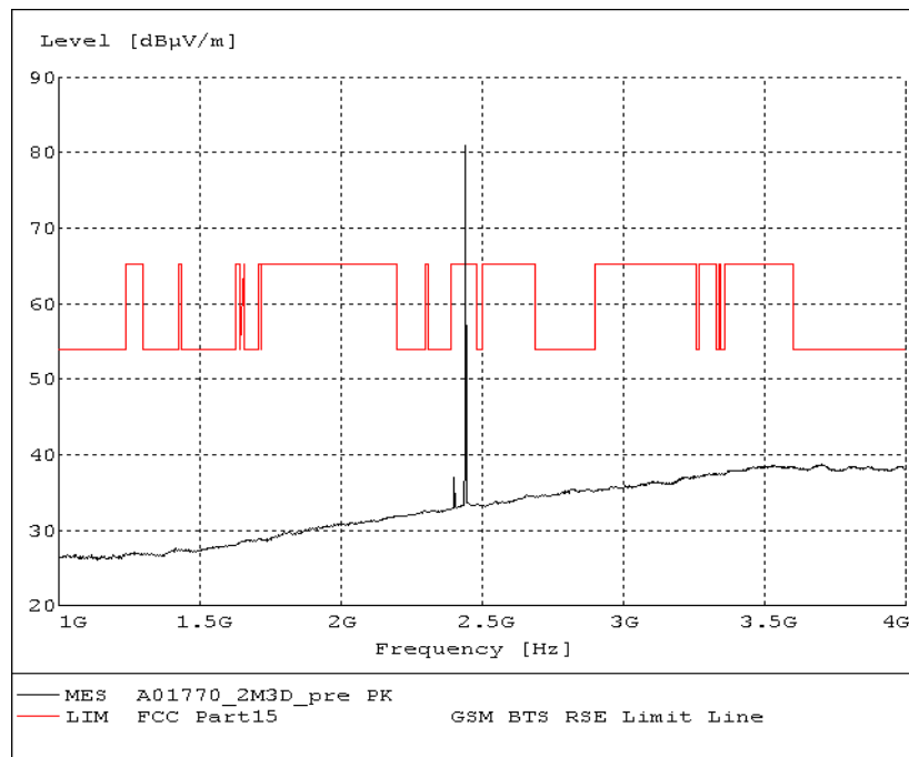
Fig.68. Radiated emission: 8DPSK, Channel 39, 1 GHz - 4 GHz
