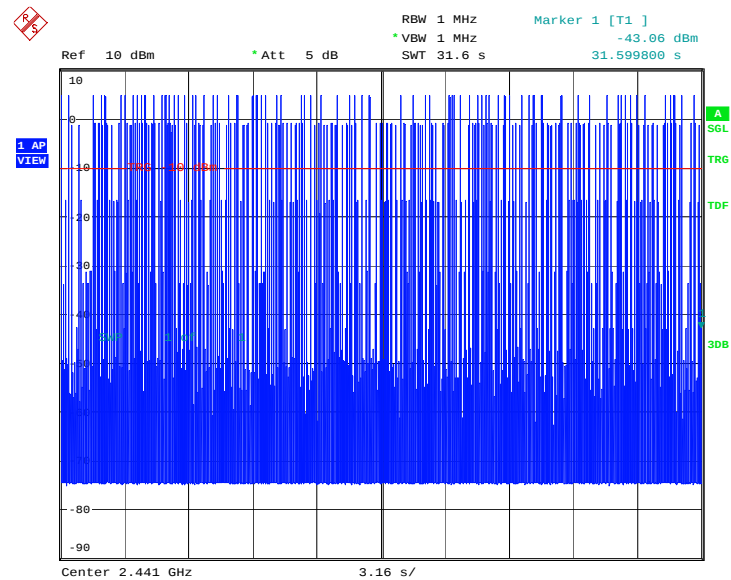
Fig.86 Time of occupancy (Dwell Time): Channel 39, Packet 2-DH5
