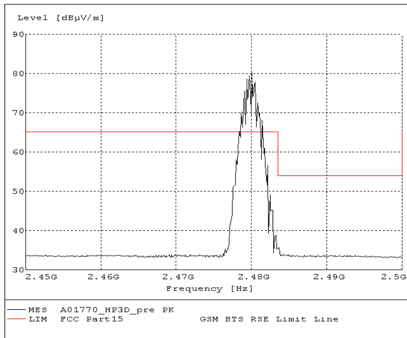
Fig.74. Radiated emission (Power): 8DPSK, high channel
