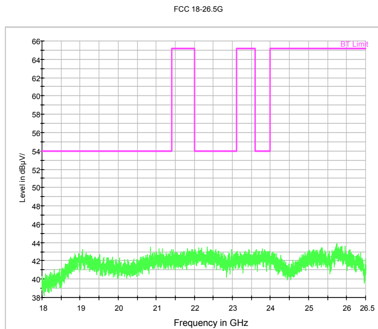
Fig.75. Radiated emission: 8DPSK, 18 GHz - 26 GHz
