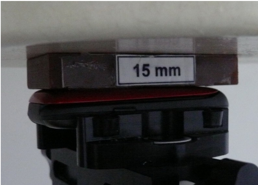
Picture 12: Body, The EUT display towards phantom, the distance from handset to the bottom of the Phantom is 15mm (The spacer was removed during testing, Close)
