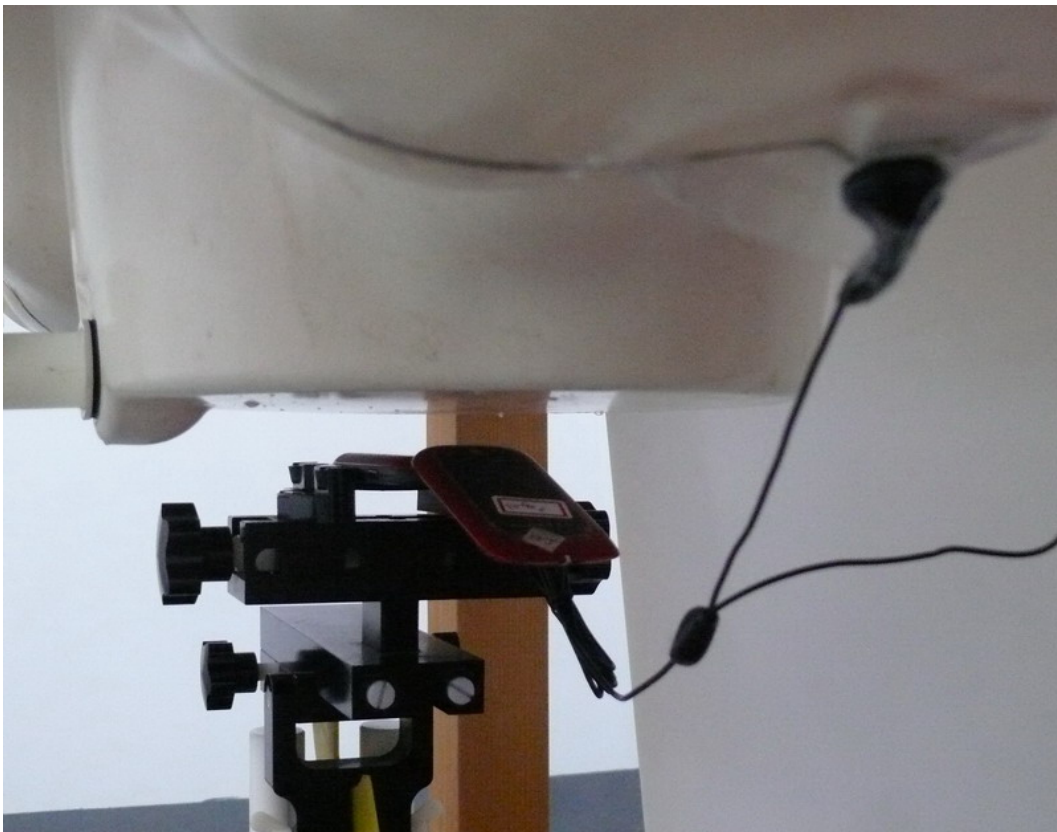
Picture 13: Body with earphone, The EUT display towards ground, the distance from handset to the bottom of the Phantom is 15mm (Open)
