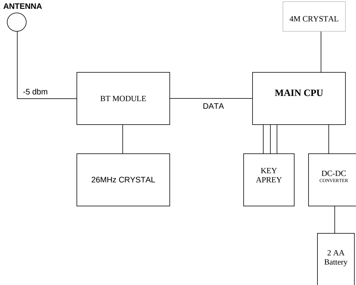
Block Diagram of BT Key-Board (2.4GHZ Transmitter) Frequency Tolerance : 2.402GHZ~2.480GHZ
