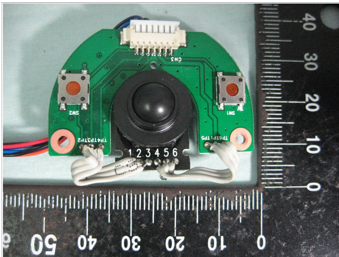
Front View of PCB Board-3
