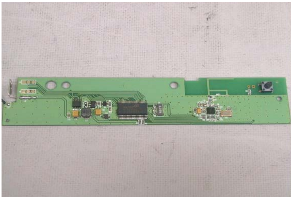
PHOTO. 6. EUT (TX) COMPONENT VIEW
