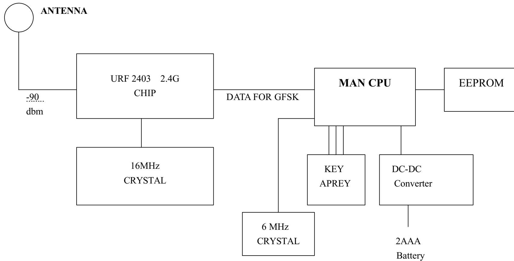
WIRELESS KEYBOARD (TX) BLOCK DIAGRAM
