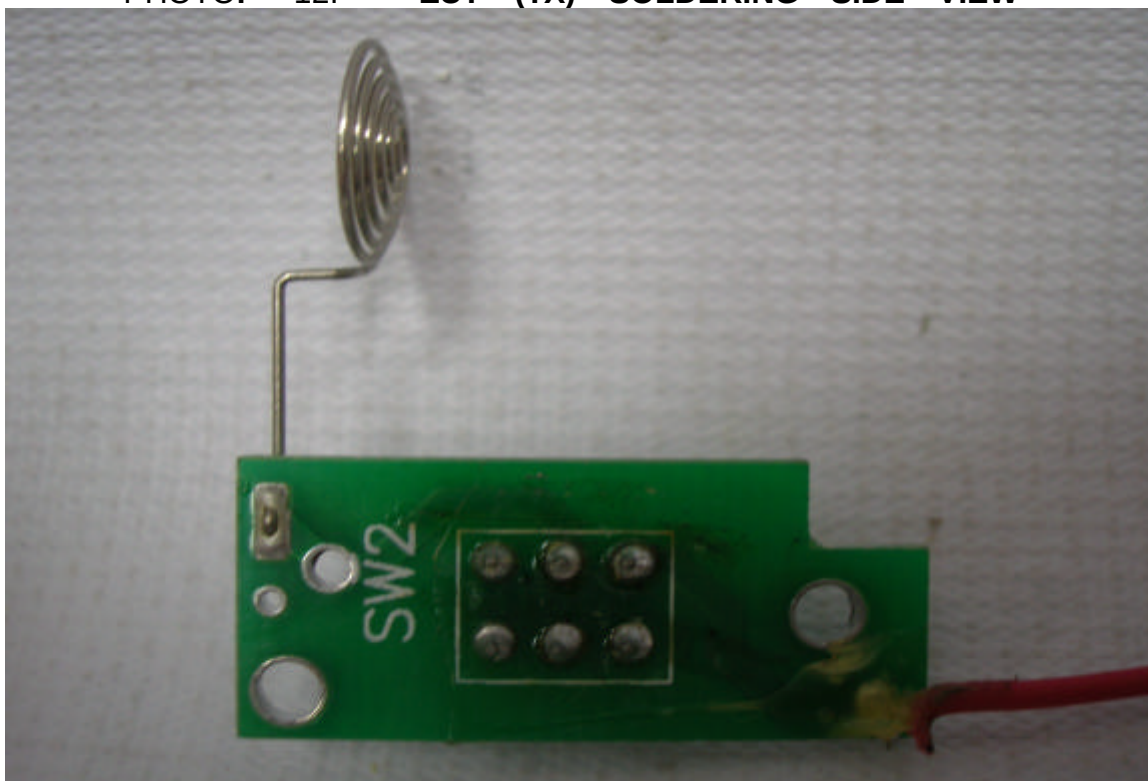
PHOTO. 12. EUT (TX) SOLDERING SIDE VIEW
