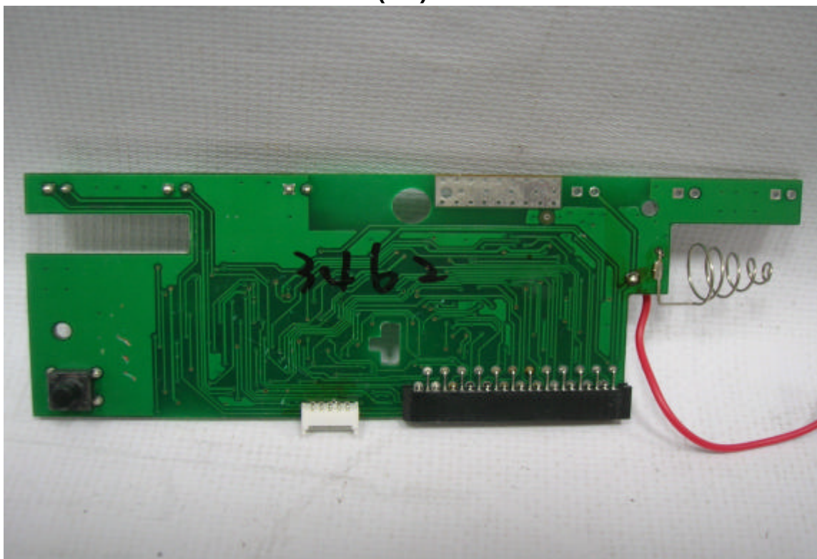
PHOTO. 10. EUT (TX) SOLDERING SIDE VIEW
