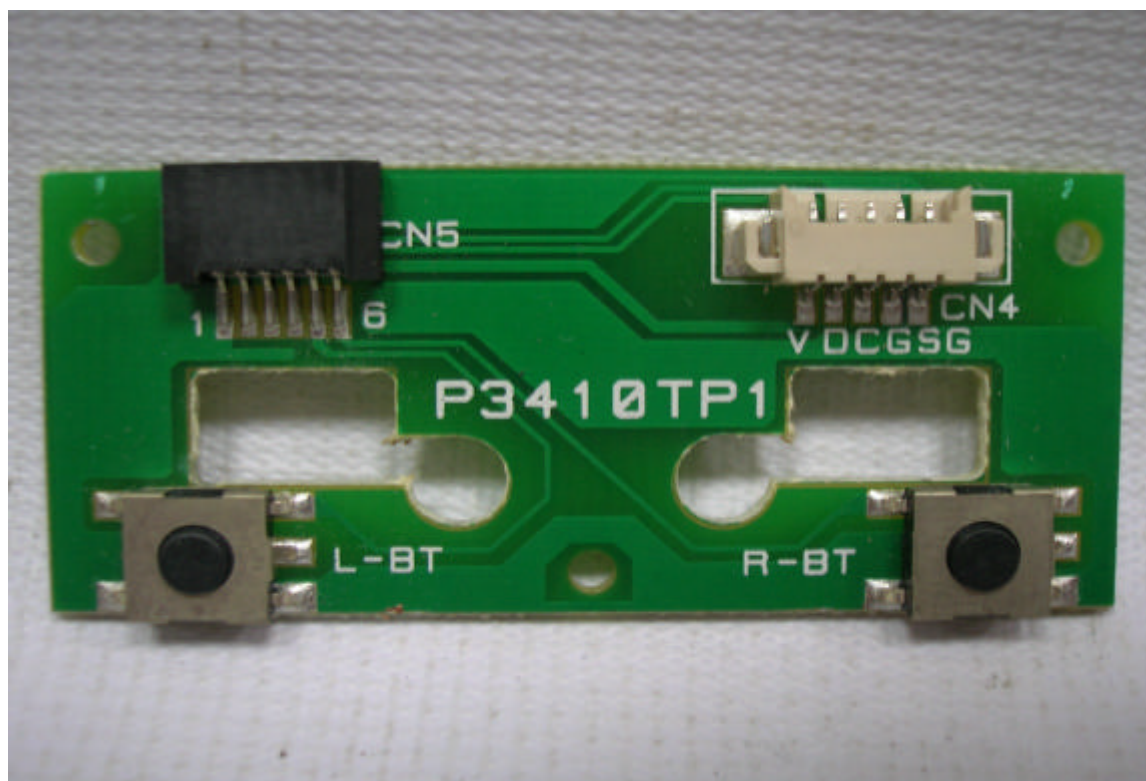
PHOTO. 16. EUT (TX) SOLDERING SIDE VIEW
