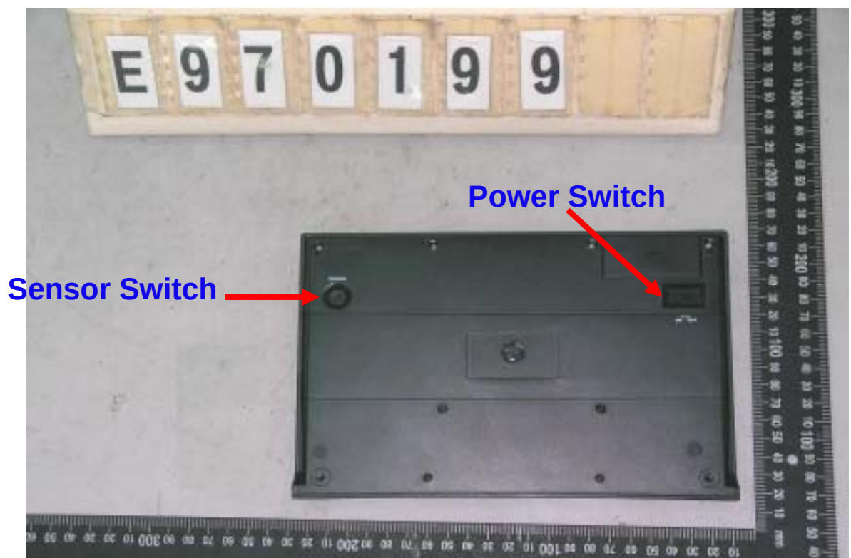
EUT REAR VIEW
